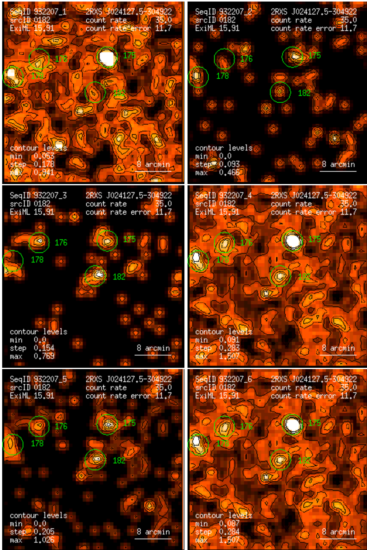
Figure 182: RASS 932207: detection 0182: band rate images, Gaussian filter: (1) PSPC channels 11 – 41, (2) 52 – 90, (3) 91 – 201, (4) 11 – 235, (5) 52 – 201, (6) 11 – 201. Broad band rates in counts/ks. Band rate contour levels in counts/ks/arcmin 2 .
