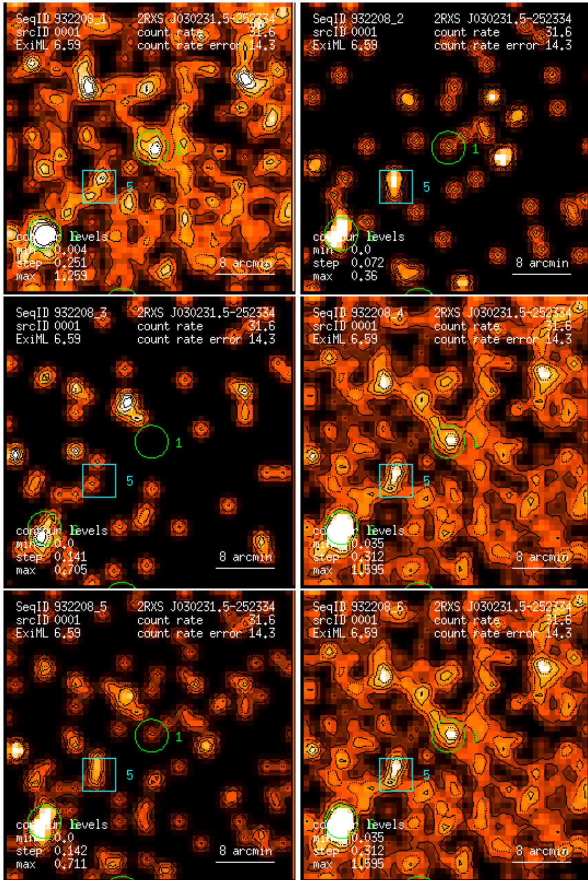
Figure 1: RASS 932208: detection 0001: band rate images, Gaussian filter: (1) PSPC channels 11 – 41, (2) 52 – 90, (3) 91 – 201, (4) 11 – 235, (5) 52 – 201, (6) 11 – 201. Broad band rates in counts/ks. Band rate contour levels in counts/ks/arcmin 2 .
