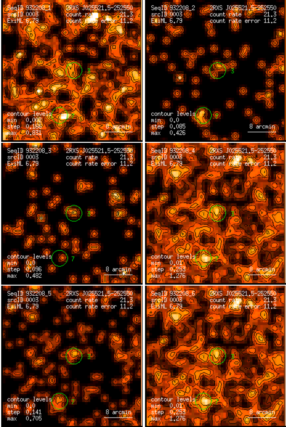
Figure 3: RASS 932208: detection 0003: band rate images, Gaussian filter: (1) PSPC channels 11 – 41, (2) 52 – 90, (3) 91 – 201, (4) 11 – 235, (5) 52 – 201, (6) 11 – 201. Broad band rates in counts/ks. Band rate contour levels in counts/ks/arcmin 2 .
