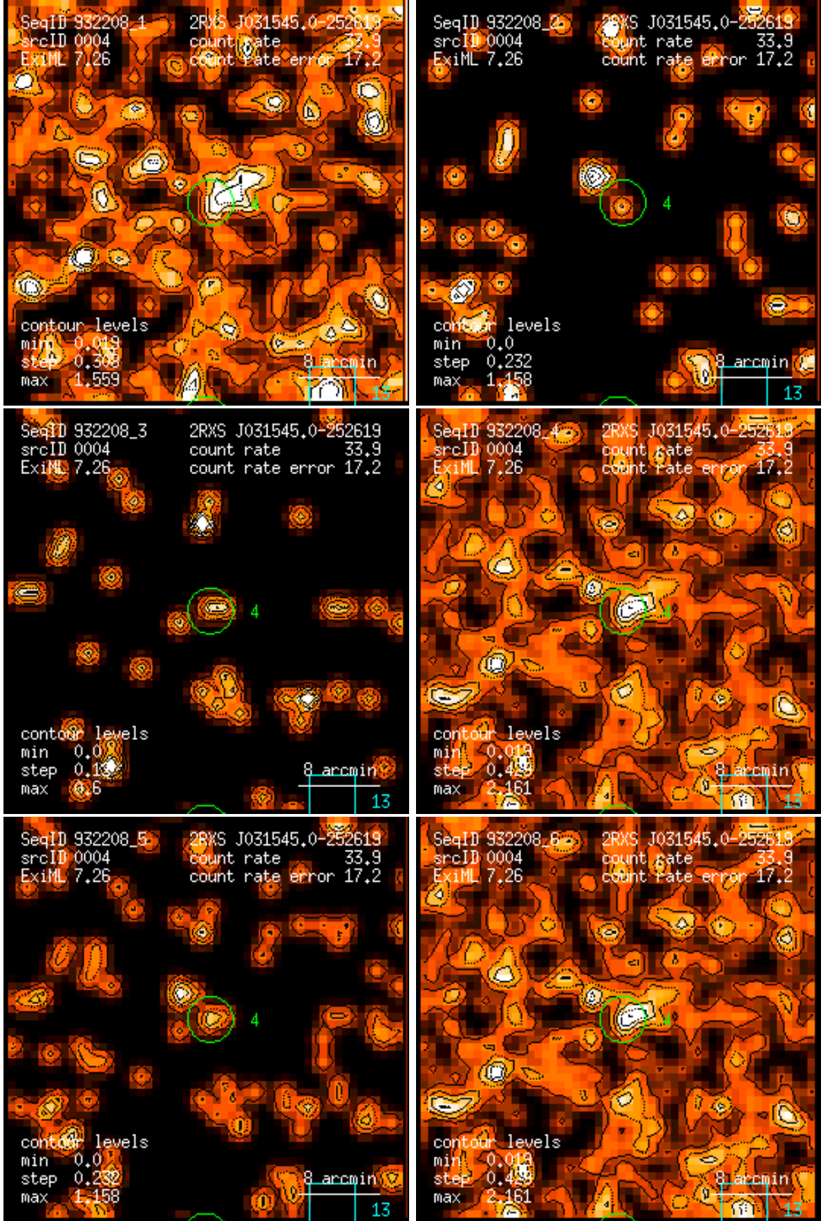
Figure 4: RASS 932208: detection 0004: band rate images, Gaussian filter: (1) PSPC channels 11 – 41, (2) 52 – 90, (3) 91 – 201, (4) 11 – 235, (5) 52 – 201, (6) 11 – 201. Broad band rates in counts/ks. Band rate contour levels in counts/ks/arcmin 2 .
