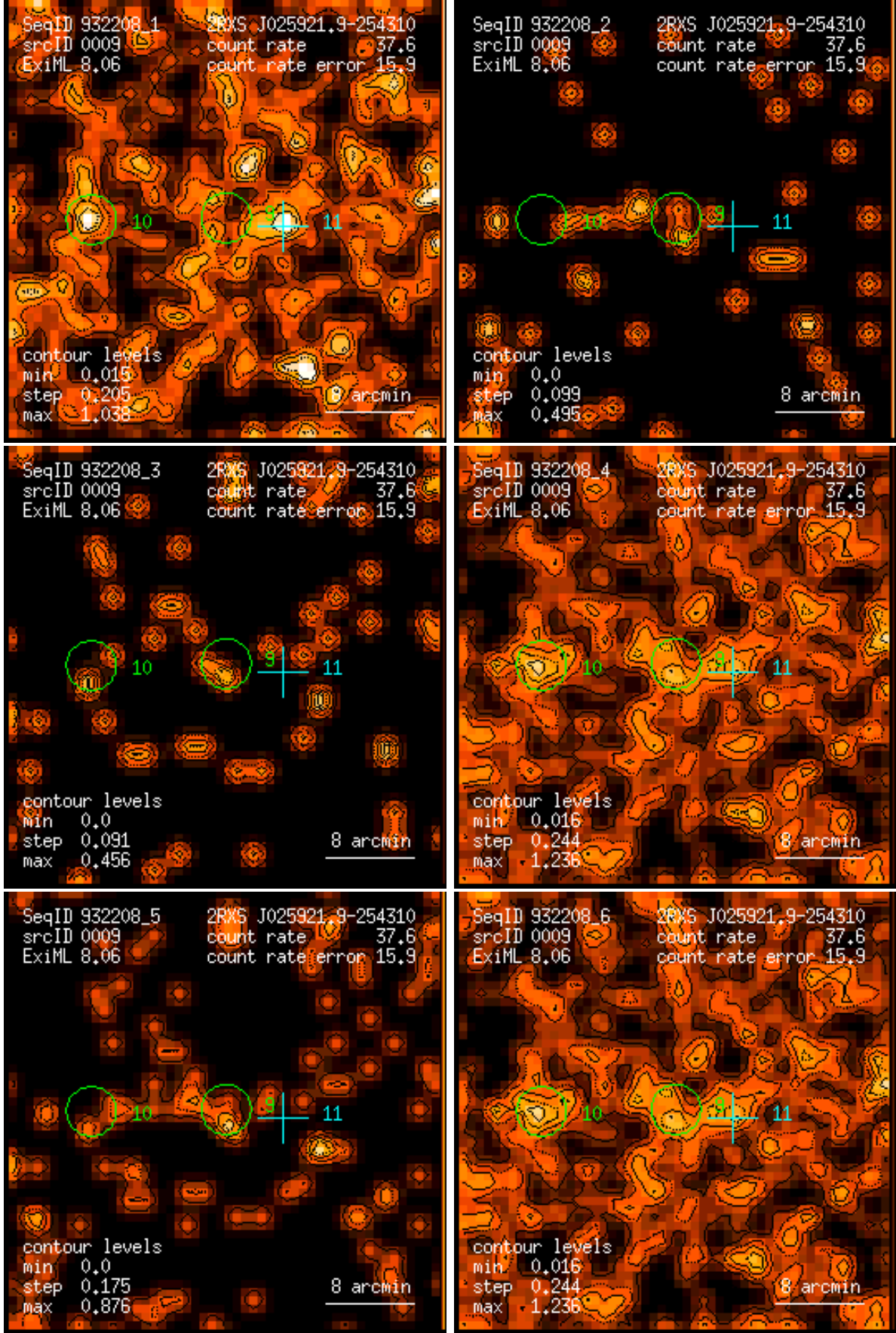
Figure 9: RASS 932208: detection 0009: band rate images, Gaussian filter: (1) PSPC channels 11 – 41, (2) 52 – 90, (3) 91 – 201, (4) 11 – 235, (5) 52 – 201, (6) 11 – 201. Broad band rates in counts/ks. Band rate contour levels in counts/ks/arcmin 2 .
