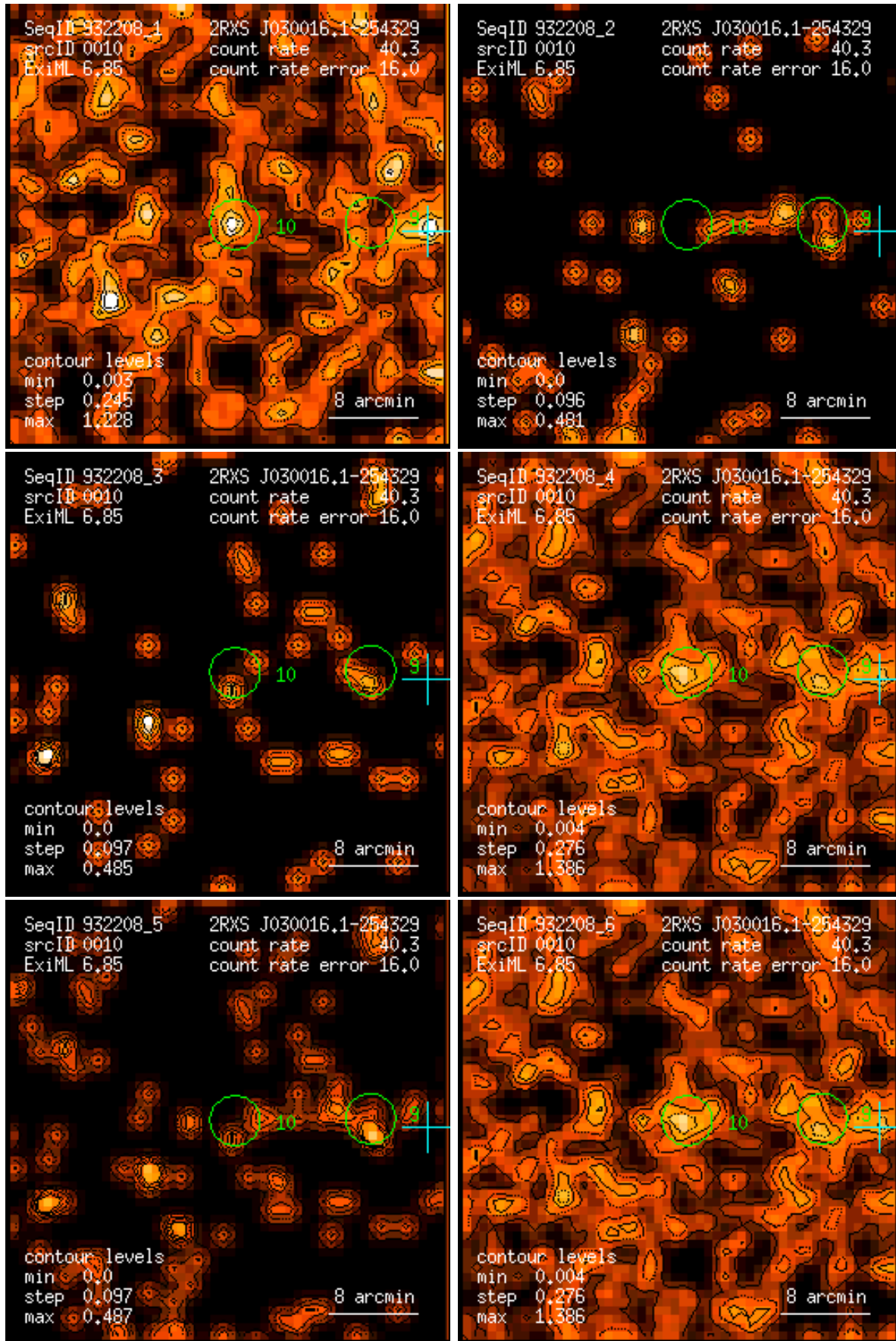
Figure 10: RASS 932208: detection 0010: band rate images, Gaussian filter: (1) PSPC channels 11 – 41, (2) 52 – 90, (3) 91 – 201, (4) 11 – 235, (5) 52 – 201, (6) 11 – 201. Broad band rates in counts/ks. Band rate contour levels in counts/ks/arcmin 2 .
