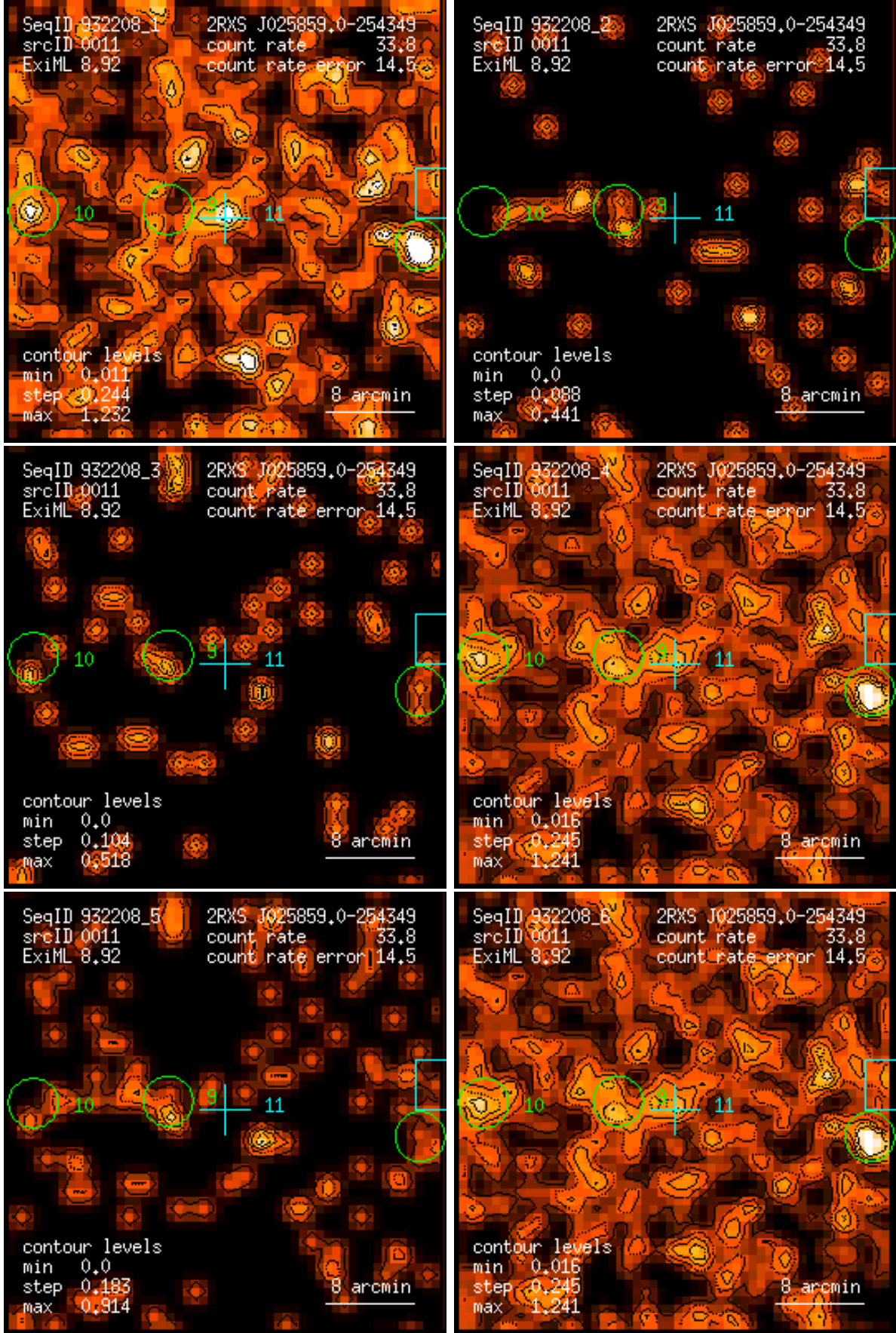
Figure 11: RASS 932208: detection 0011: band rate images, Gaussian filter: (1) PSPC channels 11 – 41, (2) 52 – 90, (3) 91 – 201, (4) 11 – 235, (5) 52 – 201, (6) 11 – 201. Broad band rates in counts/ks. Band rate contour levels in counts/ks/arcmin 2 .
