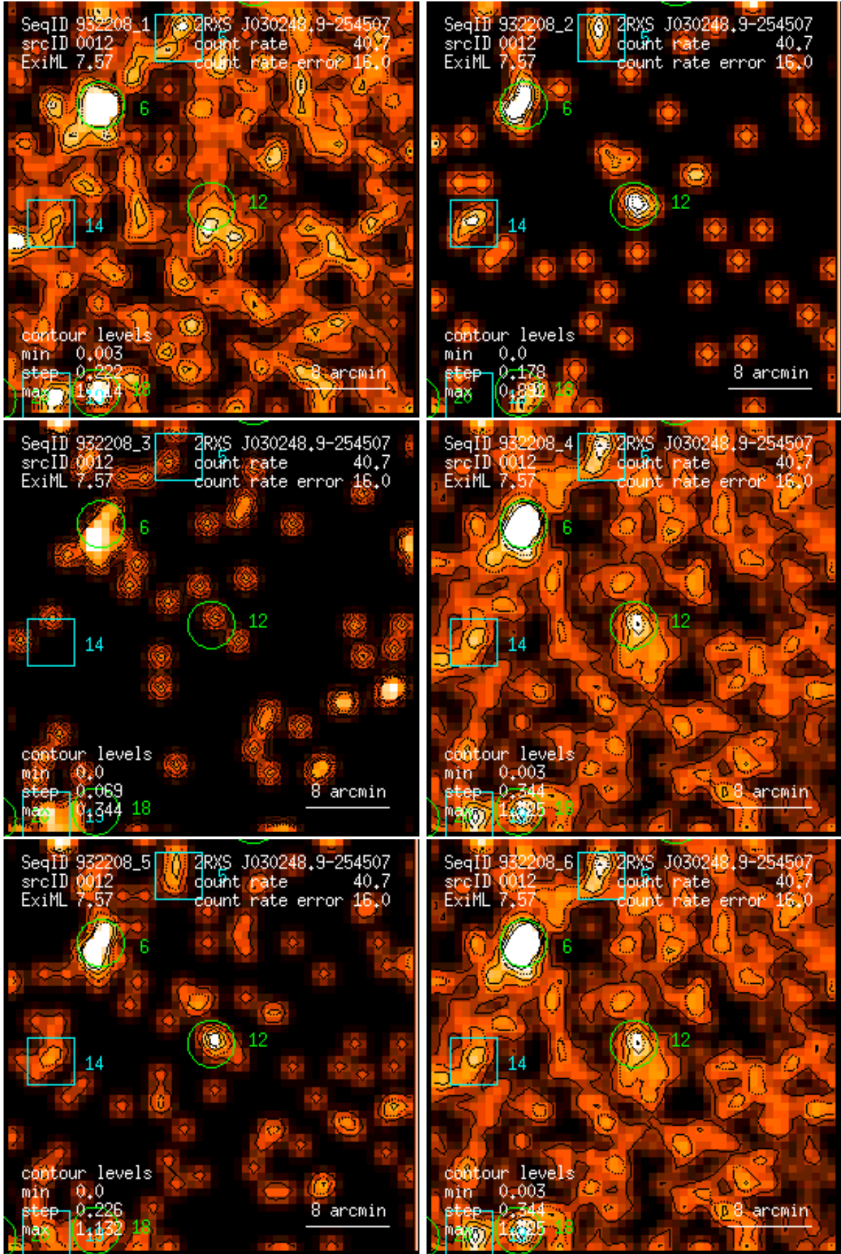
Figure 12: RASS 932208: detection 0012: band rate images, Gaussian filter: (1) PSPC channels 11 – 41, (2) 52 – 90, (3) 91 – 201, (4) 11 – 235, (5) 52 – 201, (6) 11 – 201. Broad band rates in counts/ks. Band rate contour levels in counts/ks/arcmin 2 .
