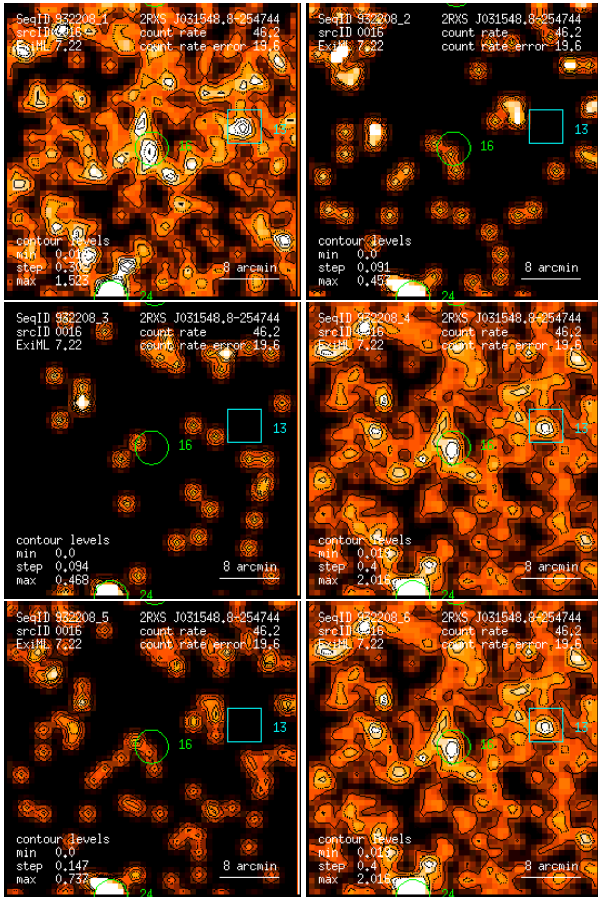
Figure 16: RASS 932208: detection 0016: band rate images, Gaussian filter: (1) PSPC channels 11 – 41, (2) 52 – 90, (3) 91 – 201, (4) 11 – 235, (5) 52 – 201, (6) 11 – 201. Broad band rates in counts/ks. Band rate contour levels in counts/ks/arcmin 2 .
