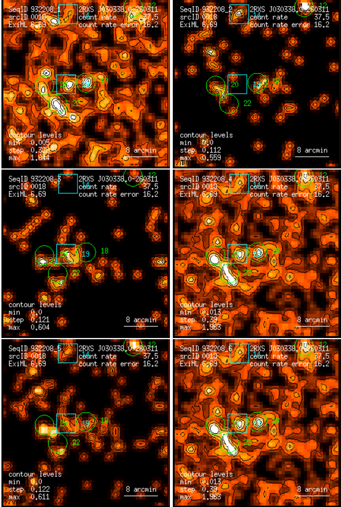
Figure 18: RASS 932208: detection 0018: band rate images, Gaussian filter: (1) PSPC channels 11 – 41, (2) 52 – 90, (3) 91 – 201, (4) 11 – 235, (5) 52 – 201, (6) 11 – 201. Broad band rates in counts/ks. Band rate contour levels in counts/ks/arcmin 2 .
