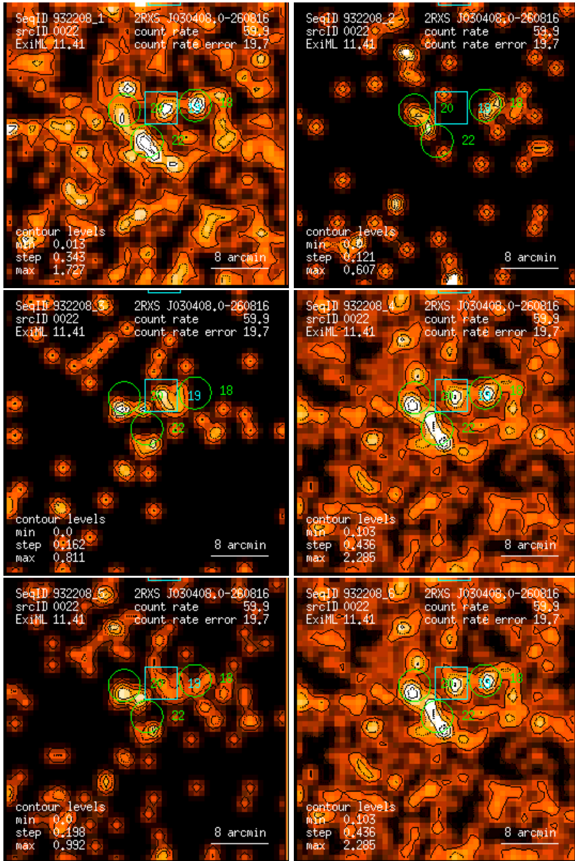
Figure 22: RASS 932208: detection 0022: band rate images, Gaussian filter: (1) PSPC channels 11 – 41, (2) 52 – 90, (3) 91 – 201, (4) 11 – 235, (5) 52 – 201, (6) 11 – 201. Broad band rates in counts/ks. Band rate contour levels in counts/ks/arcmin 2 .
