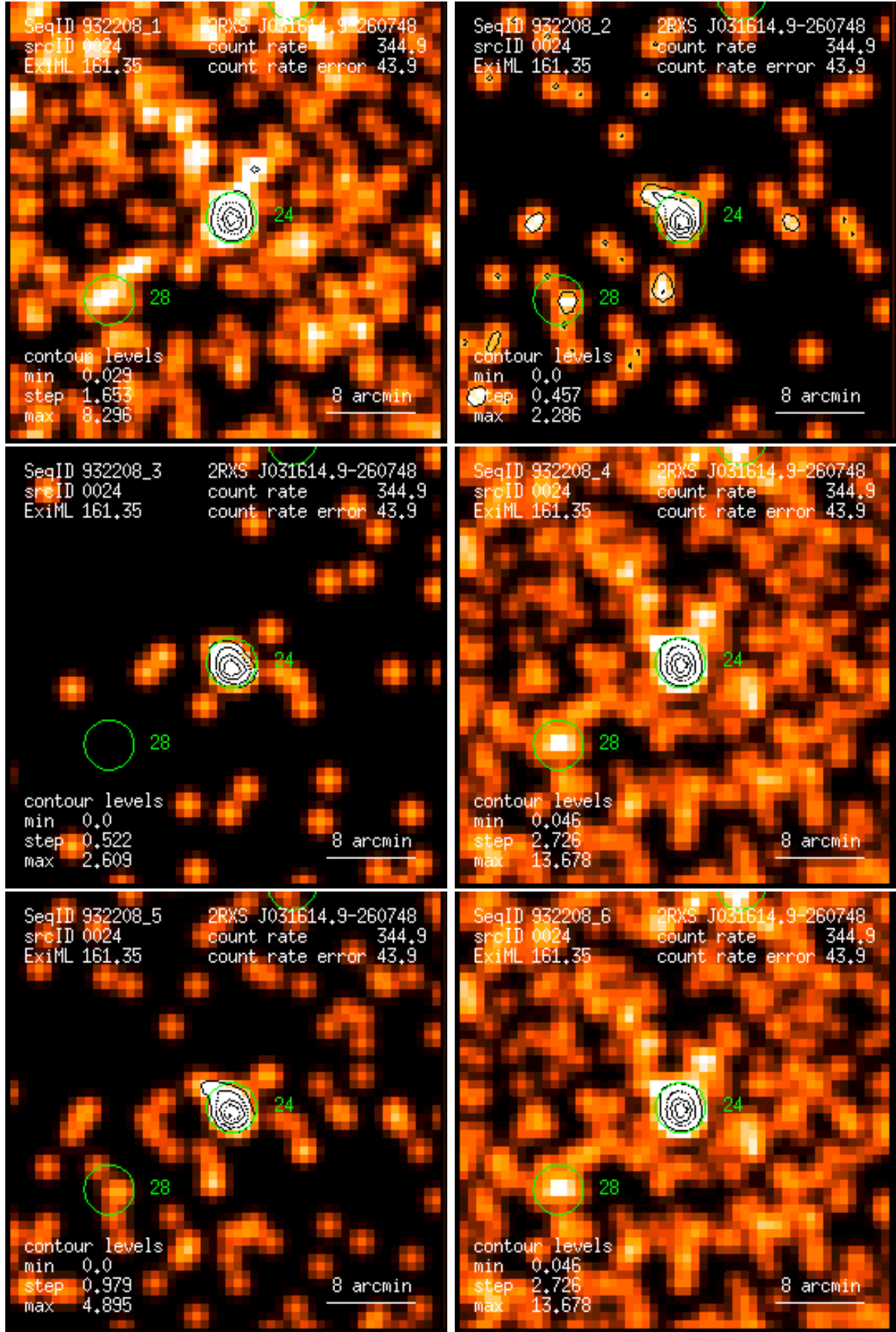
Figure 24: RASS 932208: detection 0024: band rate images, Gaussian filter: (1) PSPC channels 11 – 41, (2) 52 – 90, (3) 91 – 201, (4) 11 – 235, (5) 52 – 201, (6) 11 – 201. Broad band rates in counts/ks. Band rate contour levels in counts/ks/arcmin 2 .
