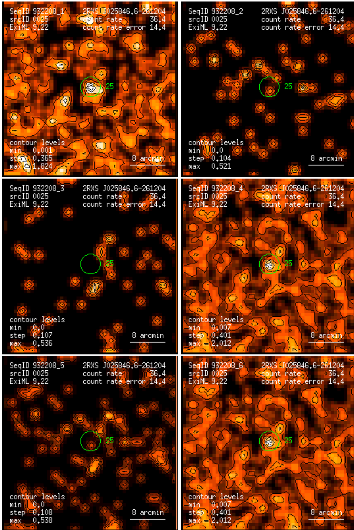
Figure 25: RASS 932208: detection 0025: band rate images, Gaussian filter: (1) PSPC channels 11 – 41, (2) 52 – 90, (3) 91 – 201, (4) 11 – 235, (5) 52 – 201, (6) 11 – 201. Broad band rates in counts/ks. Band rate contour levels in counts/ks/arcmin 2 .
