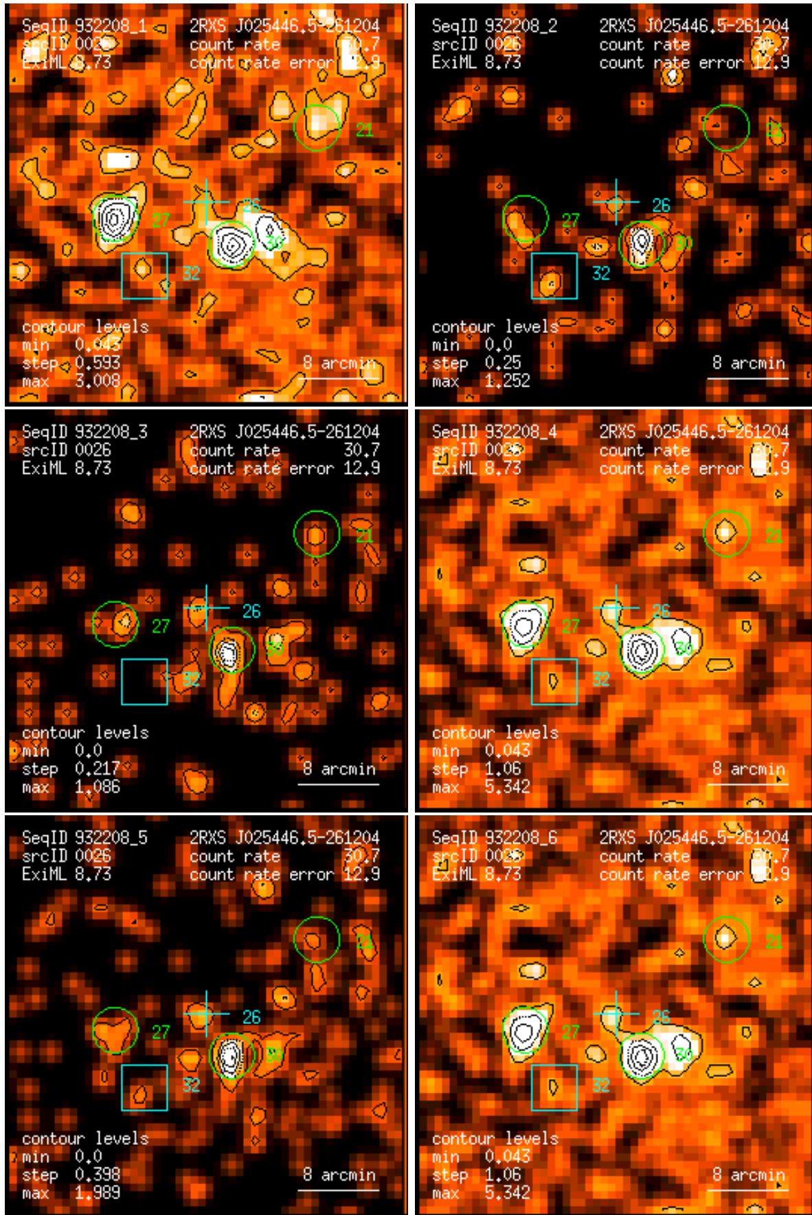
Figure 26: RASS 932208: detection 0026: band rate images, Gaussian filter: (1) PSPC channels 11 – 41, (2) 52 – 90, (3) 91 – 201, (4) 11 – 235, (5) 52 – 201, (6) 11 – 201. Broad band rates in counts/ks. Band rate contour levels in counts/ks/arcmin 2 .
