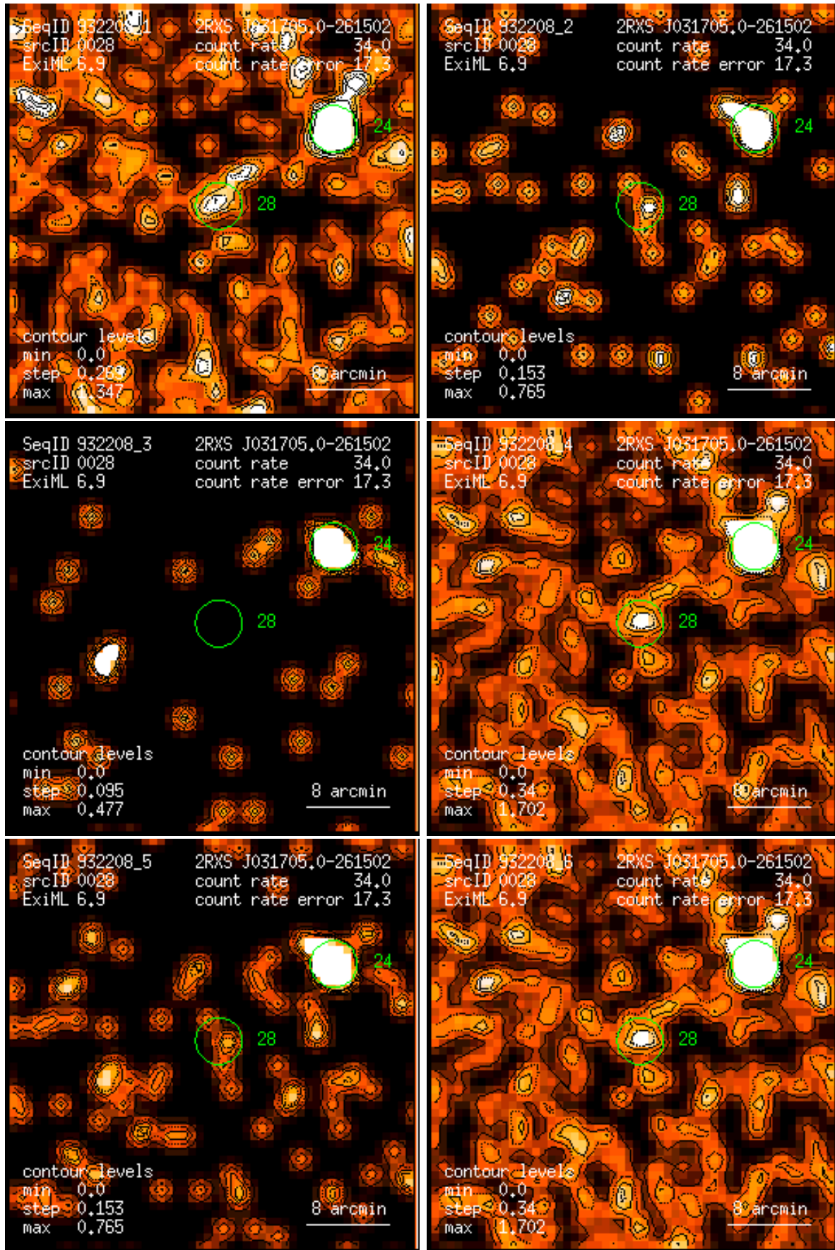
Figure 28: RASS 932208: detection 0028: band rate images, Gaussian filter: (1) PSPC channels 11 – 41, (2) 52 – 90, (3) 91 – 201, (4) 11 – 235, (5) 52 – 201, (6) 11 – 201. Broad band rates in counts/ks. Band rate contour levels in counts/ks/arcmin 2 .
