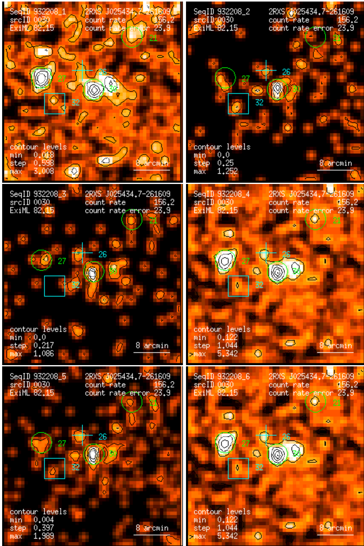
Figure 30: RASS 932208: detection 0030: band rate images, Gaussian filter: (1) PSPC channels 11 – 41, (2) 52 – 90, (3) 91 – 201, (4) 11 – 235, (5) 52 – 201, (6) 11 – 201. Broad band rates in counts/ks. Band rate contour levels in counts/ks/arcmin 2 .
