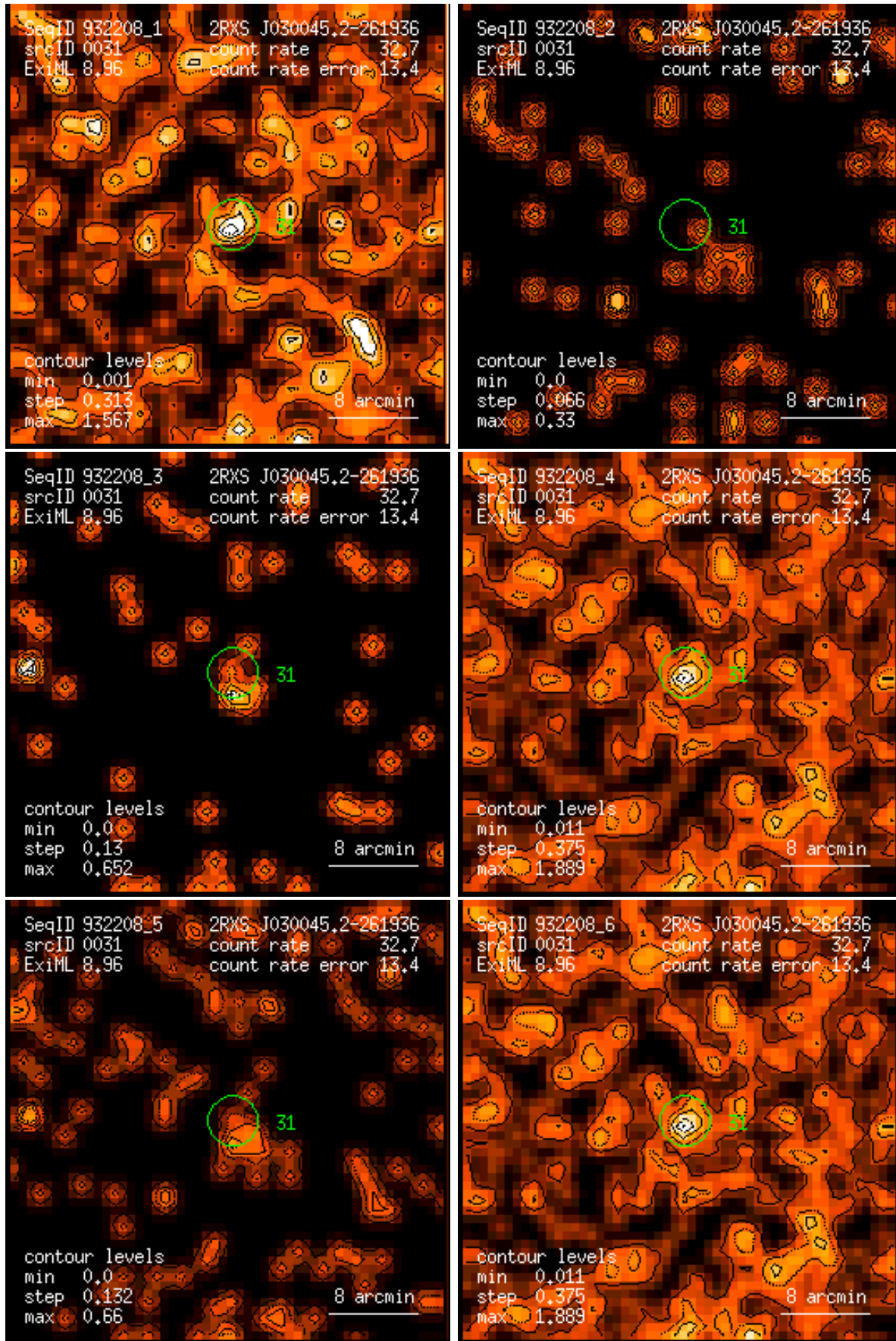
Figure 31: RASS 932208: detection 0031: band rate images, Gaussian filter: (1) PSPC channels 11 – 41, (2) 52 – 90, (3) 91 – 201, (4) 11 – 235, (5) 52 – 201, (6) 11 – 201. Broad band rates in counts/ks. Band rate contour levels in counts/ks/arcmin 2 .
