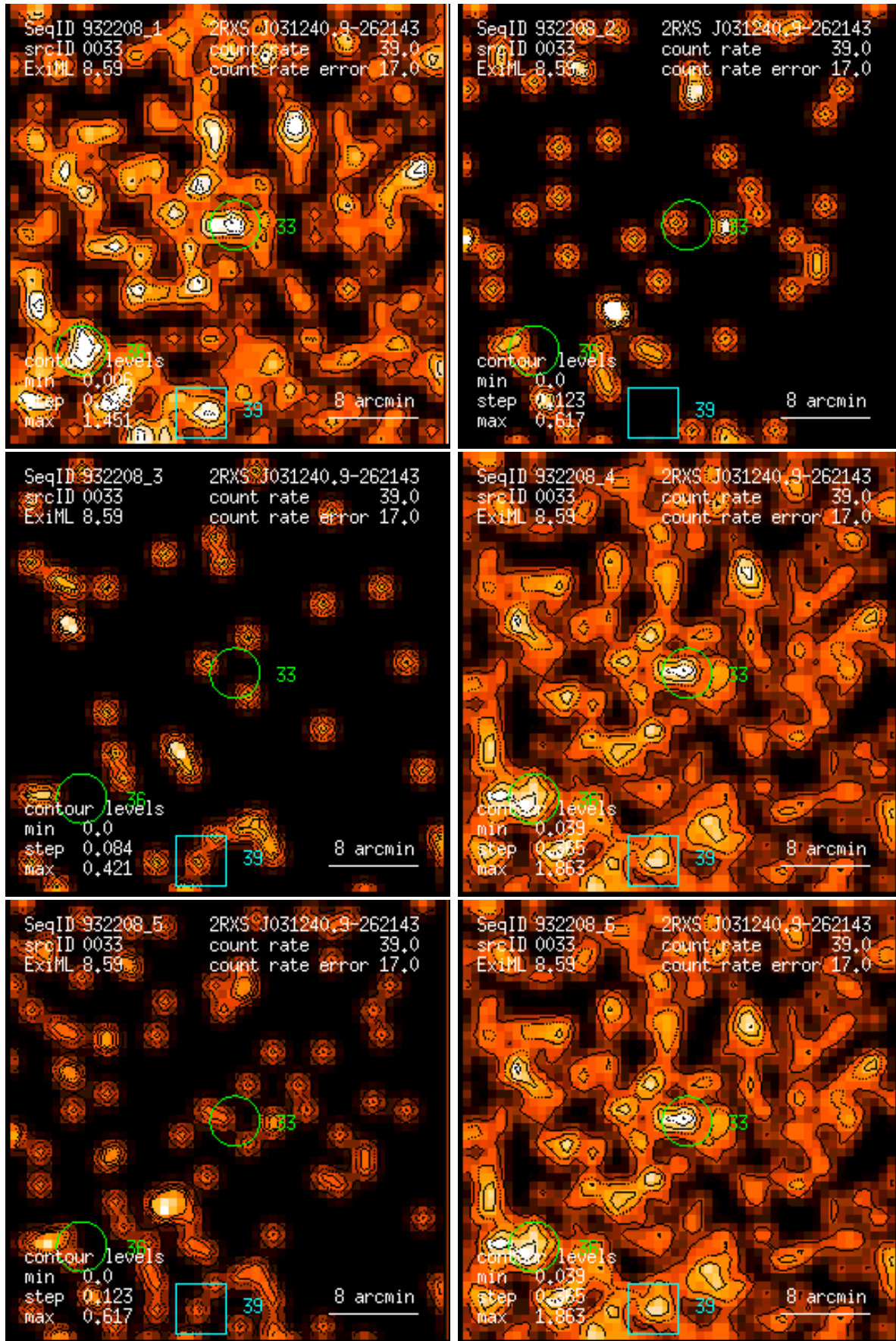
Figure 33: RASS 932208: detection 0033: band rate images, Gaussian filter: (1) PSPC channels 11 – 41, (2) 52 – 90, (3) 91 – 201, (4) 11 – 235, (5) 52 – 201, (6) 11 – 201. Broad band rates in counts/ks. Band rate contour levels in counts/ks/arcmin 2 .
