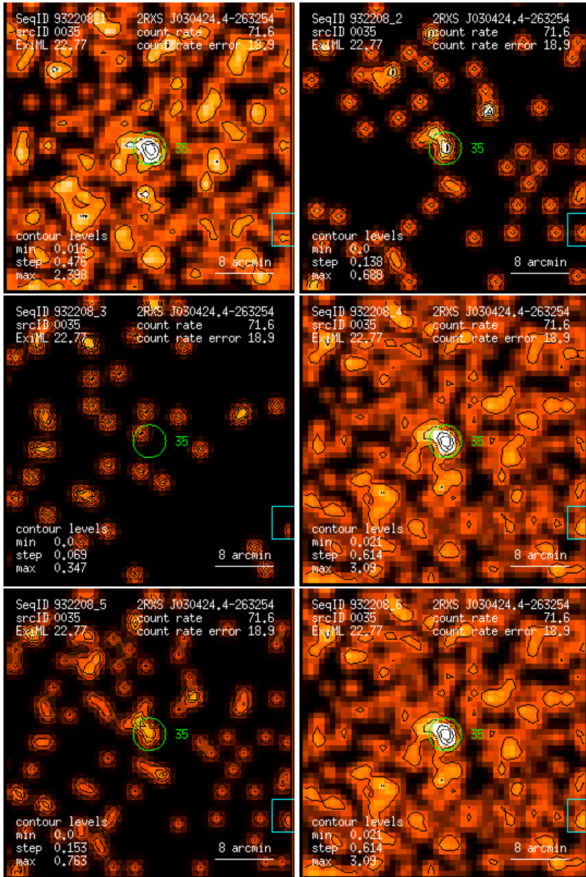
Figure 35: RASS 932208: detection 0035: band rate images, Gaussian filter: (1) PSPC channels 11 – 41, (2) 52 – 90, (3) 91 – 201, (4) 11 – 235, (5) 52 – 201, (6) 11 – 201. Broad band rates in counts/ks. Band rate contour levels in counts/ks/arcmin 2 .
