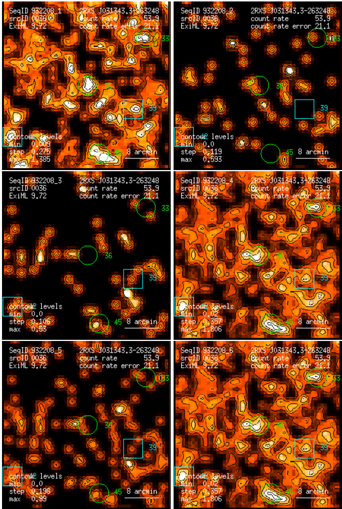
Figure 36: RASS 932208: detection 0036: band rate images, Gaussian filter: (1) PSPC channels 11 – 41, (2) 52 – 90, (3) 91 – 201, (4) 11 – 235, (5) 52 – 201, (6) 11 – 201. Broad band rates in counts/ks. Band rate contour levels in counts/ks/arcmin 2 .
