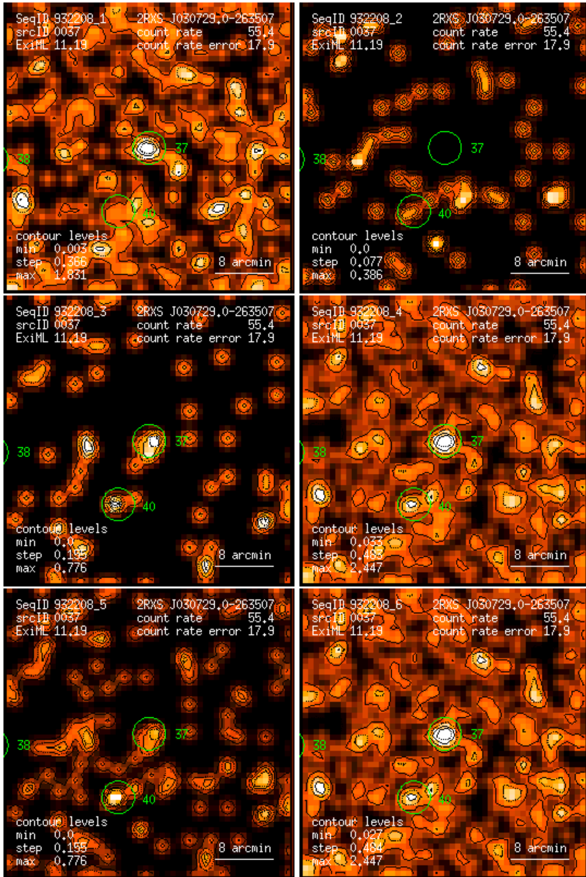
Figure 37: RASS 932208: detection 0037: band rate images, Gaussian filter: (1) PSPC channels 11 – 41, (2) 52 – 90, (3) 91 – 201, (4) 11 – 235, (5) 52 – 201, (6) 11 – 201. Broad band rates in counts/ks. Band rate contour levels in counts/ks/arcmin 2 .
