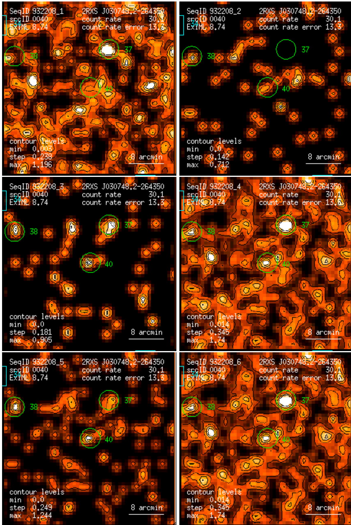
Figure 40: RASS 932208: detection 0040: band rate images, Gaussian filter: (1) PSPC channels 11 – 41, (2) 52 – 90, (3) 91 – 201, (4) 11 – 235, (5) 52 – 201, (6) 11 – 201. Broad band rates in counts/ks. Band rate contour levels in counts/ks/arcmin 2 .
