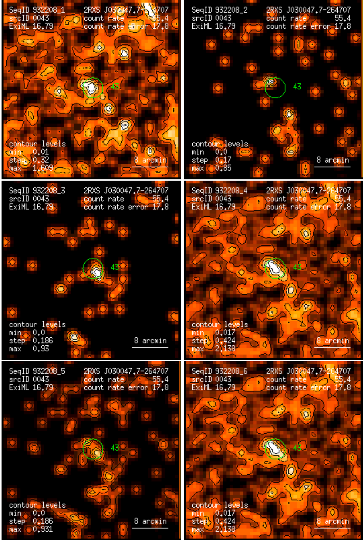
Figure 43: RASS 932208: detection 0043: band rate images, Gaussian filter: (1) PSPC channels 11 – 41, (2) 52 – 90, (3) 91 – 201, (4) 11 – 235, (5) 52 – 201, (6) 11 – 201. Broad band rates in counts/ks. Band rate contour levels in counts/ks/arcmin 2 .
