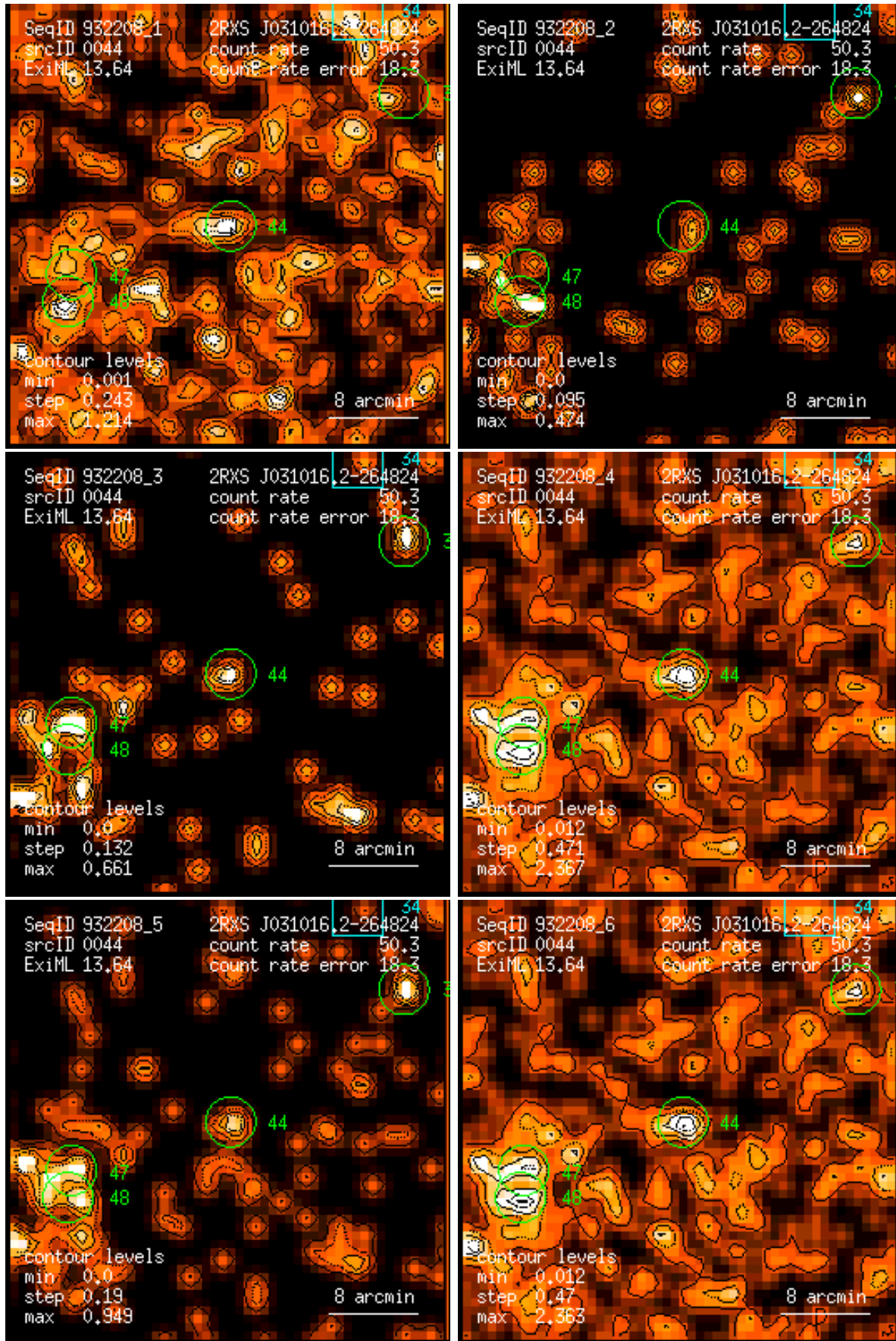
Figure 44: RASS 932208: detection 0044: band rate images, Gaussian filter: (1) PSPC channels 11 – 41, (2) 52 – 90, (3) 91 – 201, (4) 11 – 235, (5) 52 – 201, (6) 11 – 201. Broad band rates in counts/ks. Band rate contour levels in counts/ks/arcmin 2 .
