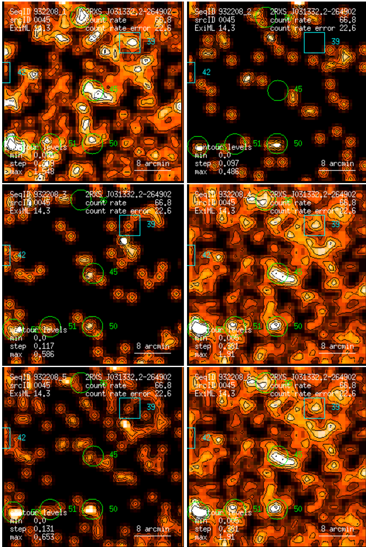
Figure 45: RASS 932208: detection 0045: band rate images, Gaussian filter: (1) PSPC channels 11 – 41, (2) 52 – 90, (3) 91 – 201, (4) 11 – 235, (5) 52 – 201, (6) 11 – 201. Broad band rates in counts/ks. Band rate contour levels in counts/ks/arcmin 2 .
