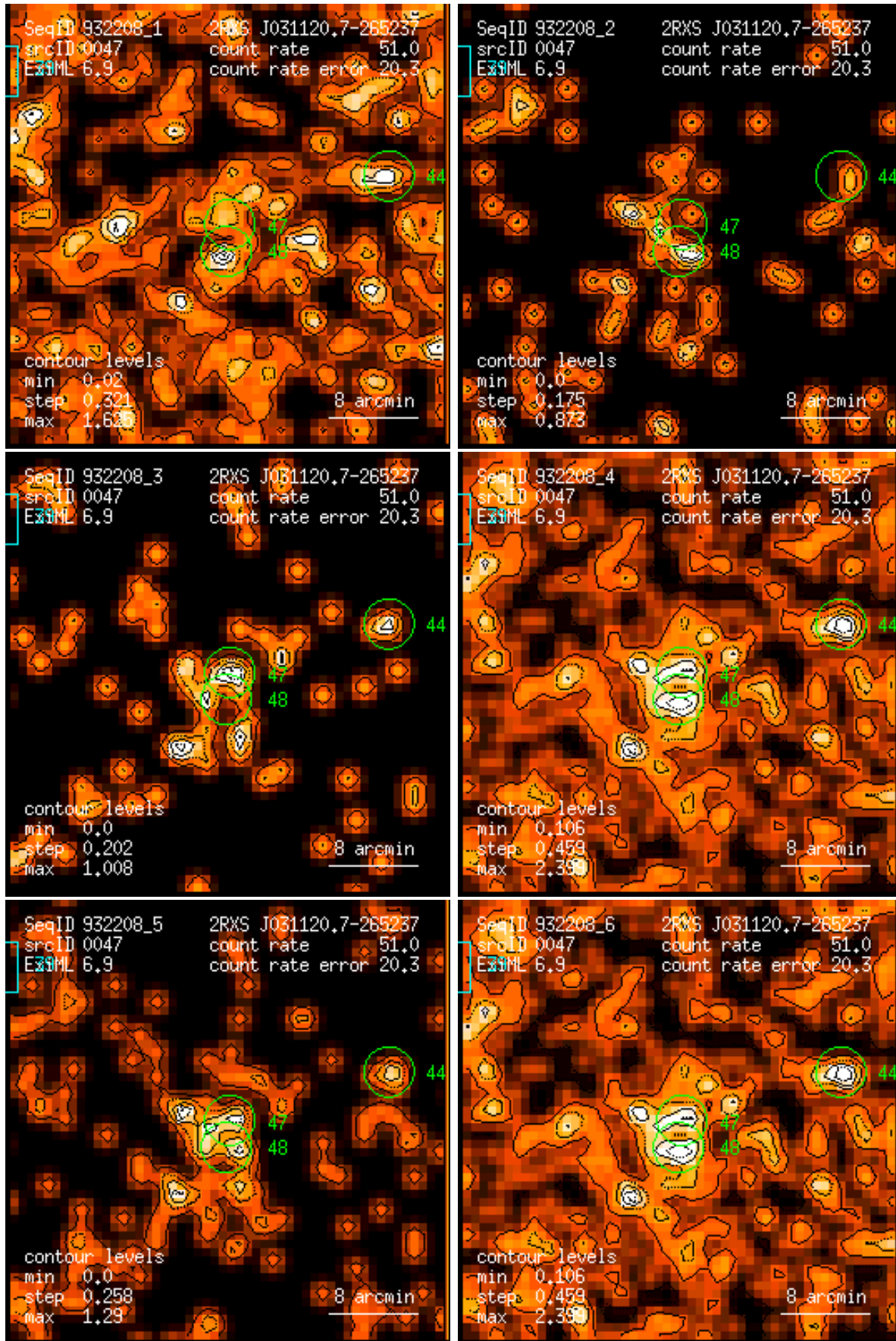
Figure 47: RASS 932208: detection 0047: band rate images, Gaussian filter: (1) PSPC channels 11 – 41, (2) 52 – 90, (3) 91 – 201, (4) 11 – 235, (5) 52 – 201, (6) 11 – 201. Broad band rates in counts/ks. Band rate contour levels in counts/ks/arcmin 2 .
