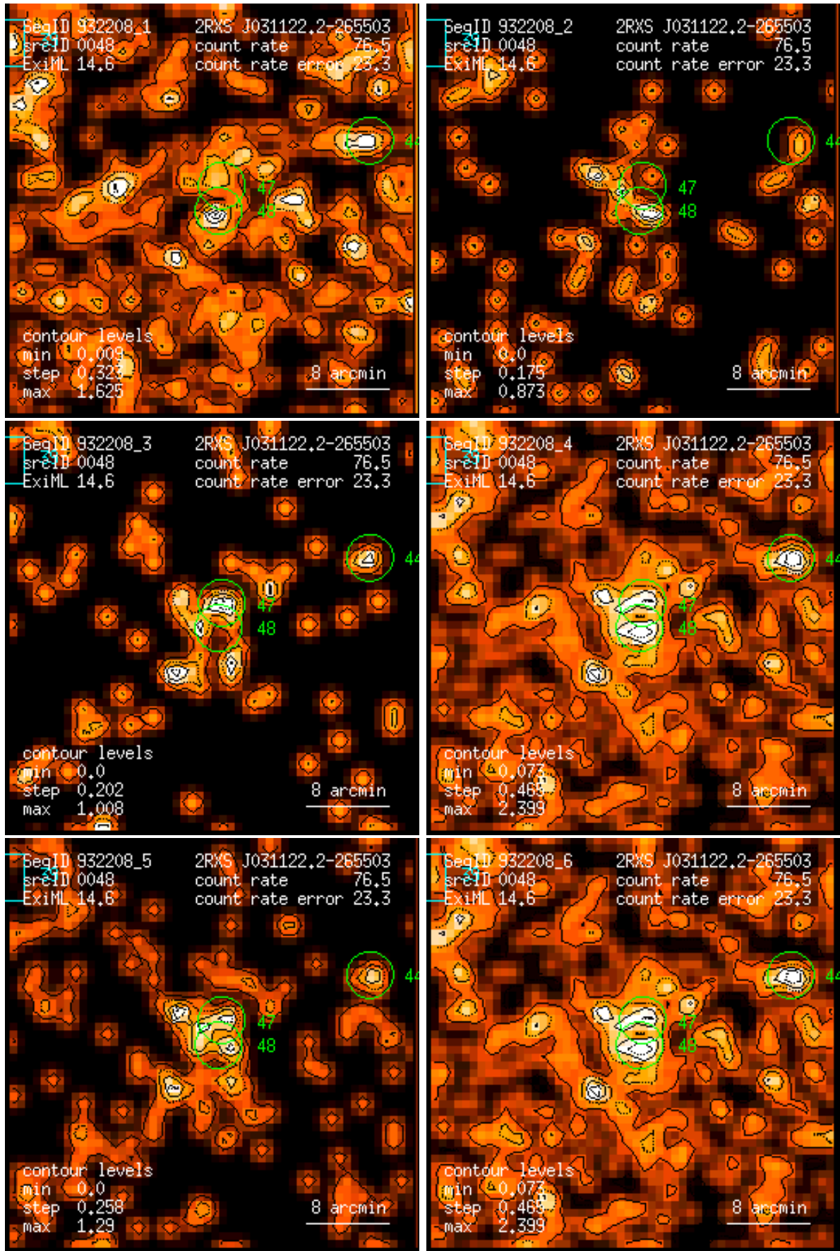
Figure 48: RASS 932208: detection 0048: band rate images, Gaussian filter: (1) PSPC channels 11 – 41, (2) 52 – 90, (3) 91 – 201, (4) 11 – 235, (5) 52 – 201, (6) 11 – 201. Broad band rates in counts/ks. Band rate contour levels in counts/ks/arcmin 2 .
