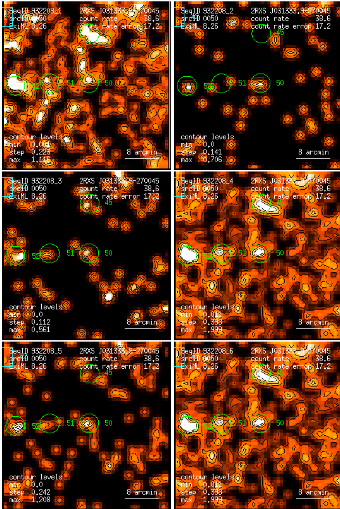
Figure 50: RASS 932208: detection 0050: band rate images, Gaussian filter: (1) PSPC channels 11 – 41, (2) 52 – 90, (3) 91 – 201, (4) 11 – 235, (5) 52 – 201, (6) 11 – 201. Broad band rates in counts/ks. Band rate contour levels in counts/ks/arcmin 2 .
