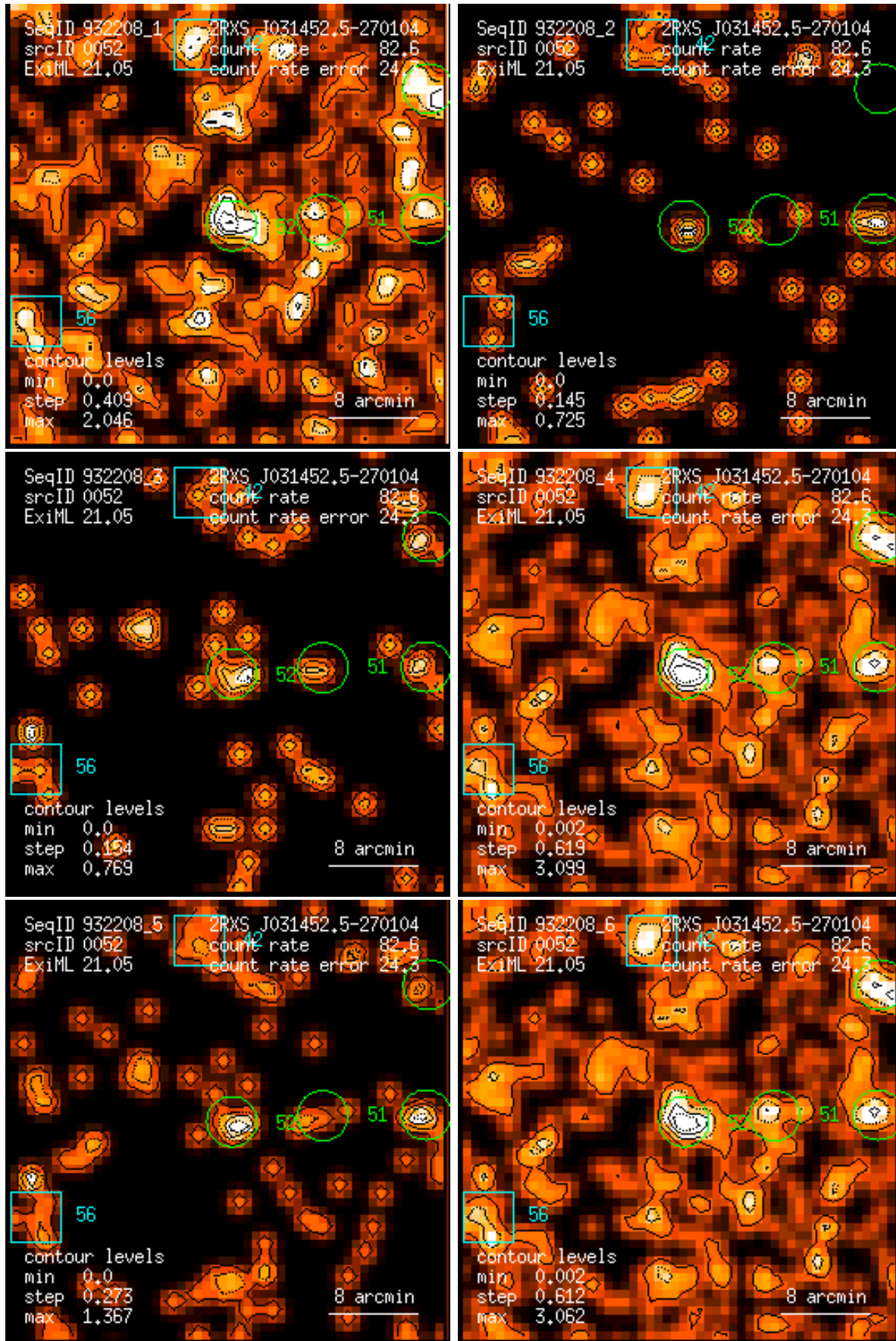
Figure 52: RASS 932208: detection 0052: band rate images, Gaussian filter: (1) PSPC channels 11 – 41, (2) 52 – 90, (3) 91 – 201, (4) 11 – 235, (5) 52 – 201, (6) 11 – 201. Broad band rates in counts/ks. Band rate contour levels in counts/ks/arcmin 2 .
