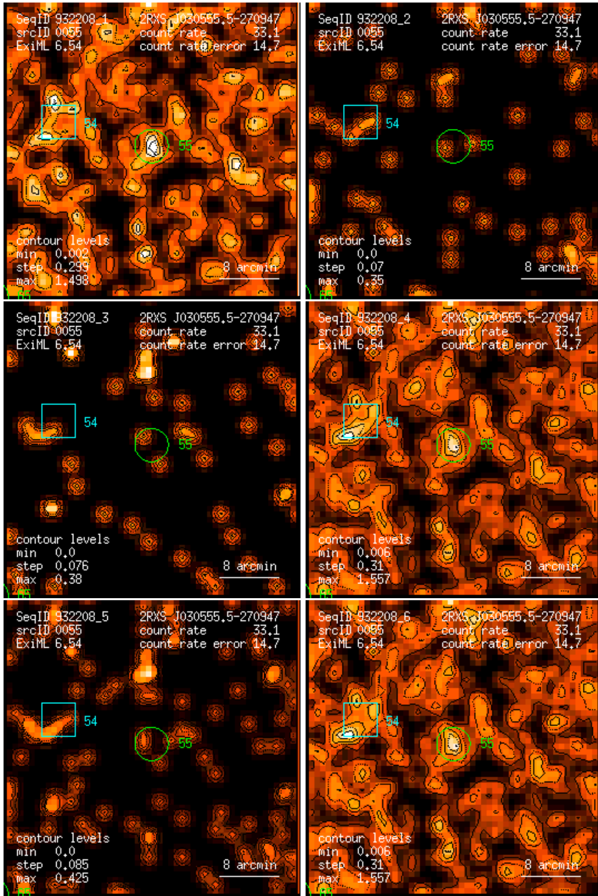
Figure 55: RASS 932208: detection 0055: band rate images, Gaussian filter: (1) PSPC channels 11 – 41, (2) 52 – 90, (3) 91 – 201, (4) 11 – 235, (5) 52 – 201, (6) 11 – 201. Broad band rates in counts/ks. Band rate contour levels in counts/ks/arcmin 2 .
