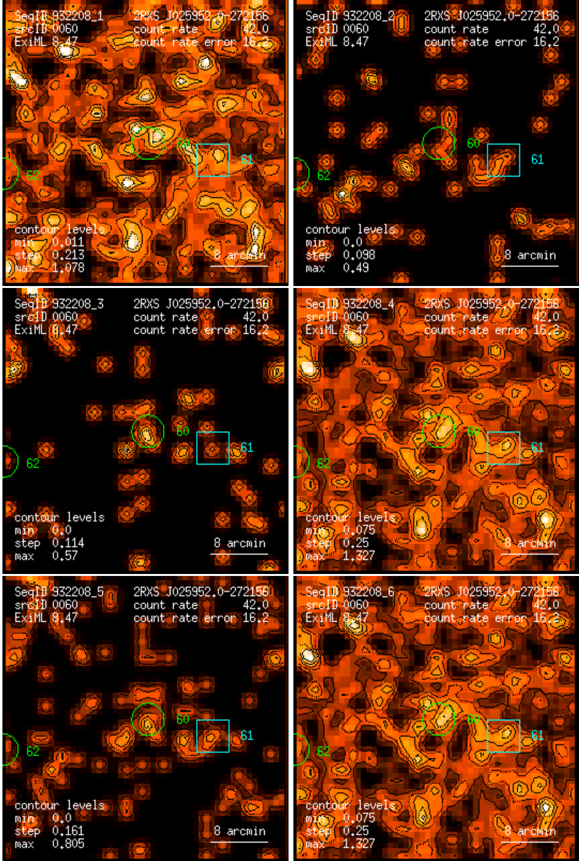
Figure 60: RASS 932208: detection 0060: band rate images, Gaussian filter: (1) PSPC channels 11 – 41, (2) 52 – 90, (3) 91 – 201, (4) 11 – 235, (5) 52 – 201, (6) 11 – 201. Broad band rates in counts/ks. Band rate contour levels in counts/ks/arcmin 2 .
