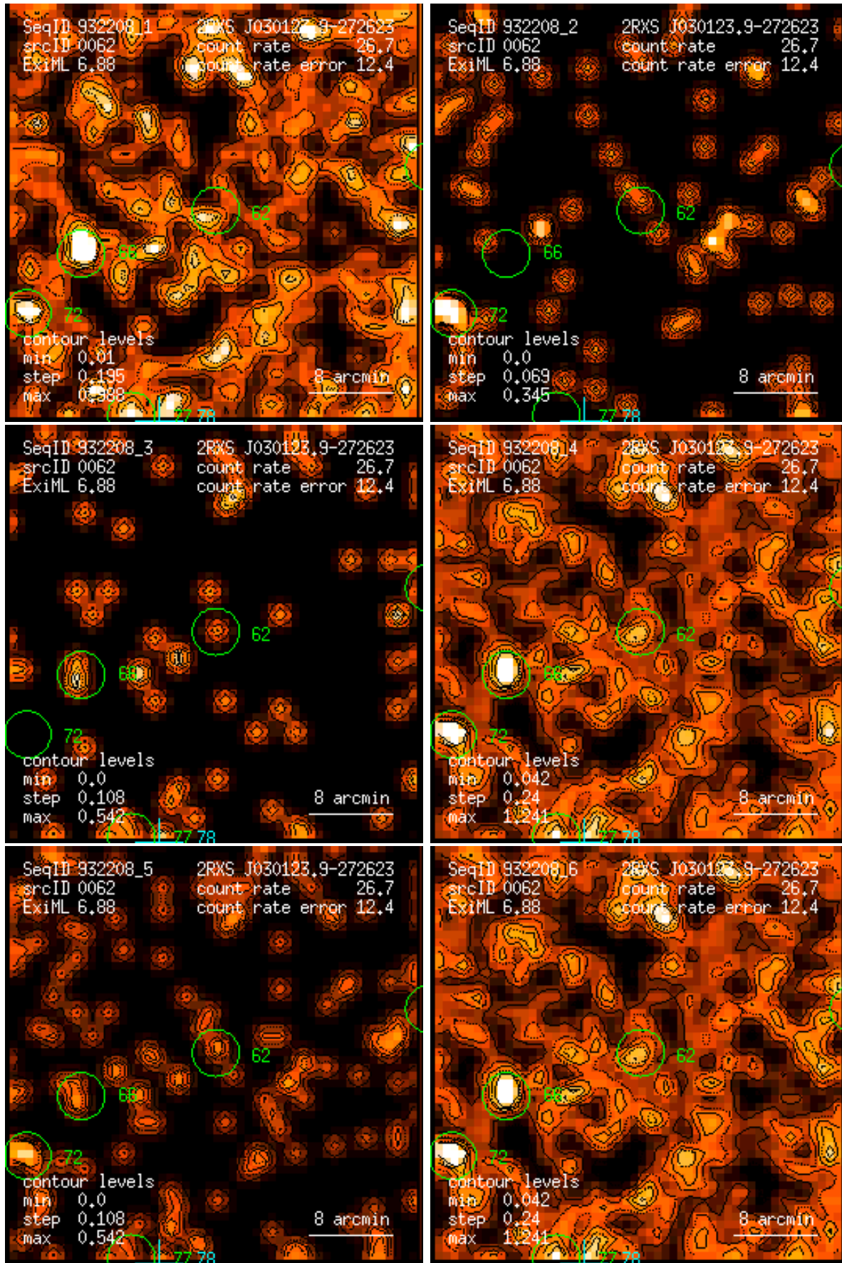
Figure 62: RASS 932208: detection 0062: band rate images, Gaussian filter: (1) PSPC channels 11 – 41, (2) 52 – 90, (3) 91 – 201, (4) 11 – 235, (5) 52 – 201, (6) 11 – 201. Broad band rates in counts/ks. Band rate contour levels in counts/ks/arcmin 2 .
