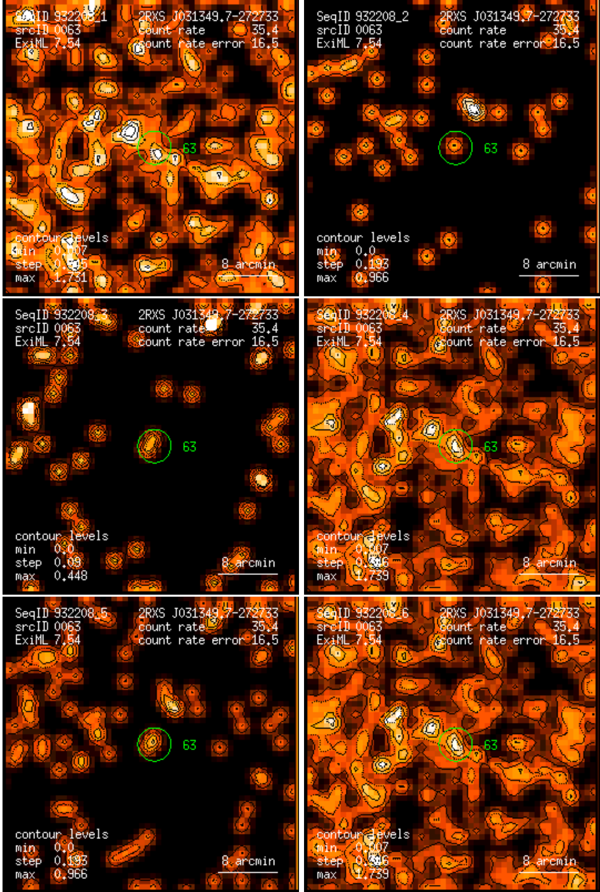
Figure 63: RASS 932208: detection 0063: band rate images, Gaussian filter: (1) PSPC channels 11 – 41, (2) 52 – 90, (3) 91 – 201, (4) 11 – 235, (5) 52 – 201, (6) 11 – 201. Broad band rates in counts/ks. Band rate contour levels in counts/ks/arcmin 2 .
