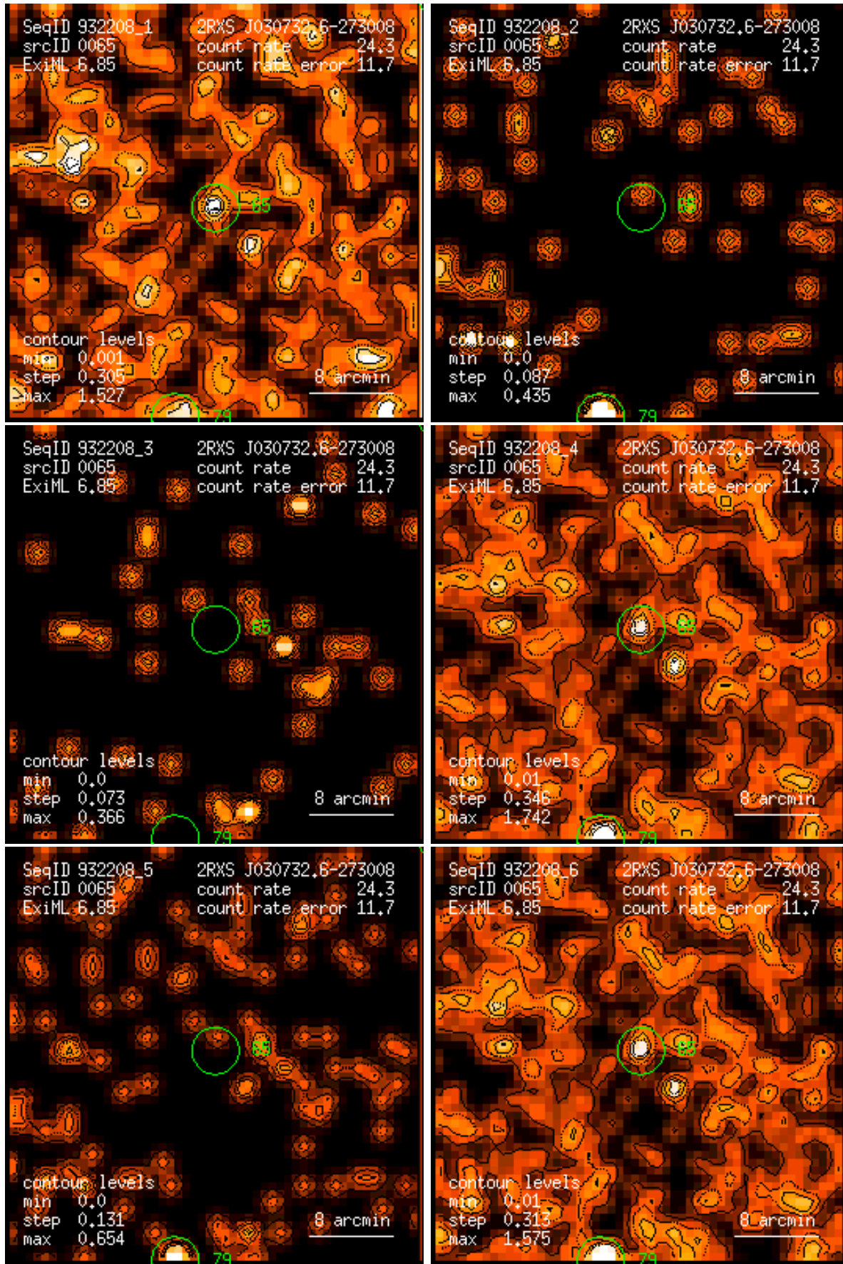
Figure 65: RASS 932208: detection 0065: band rate images, Gaussian filter: (1) PSPC channels 11 – 41, (2) 52 – 90, (3) 91 – 201, (4) 11 – 235, (5) 52 – 201, (6) 11 – 201. Broad band rates in counts/ks. Band rate contour levels in counts/ks/arcmin 2 .
