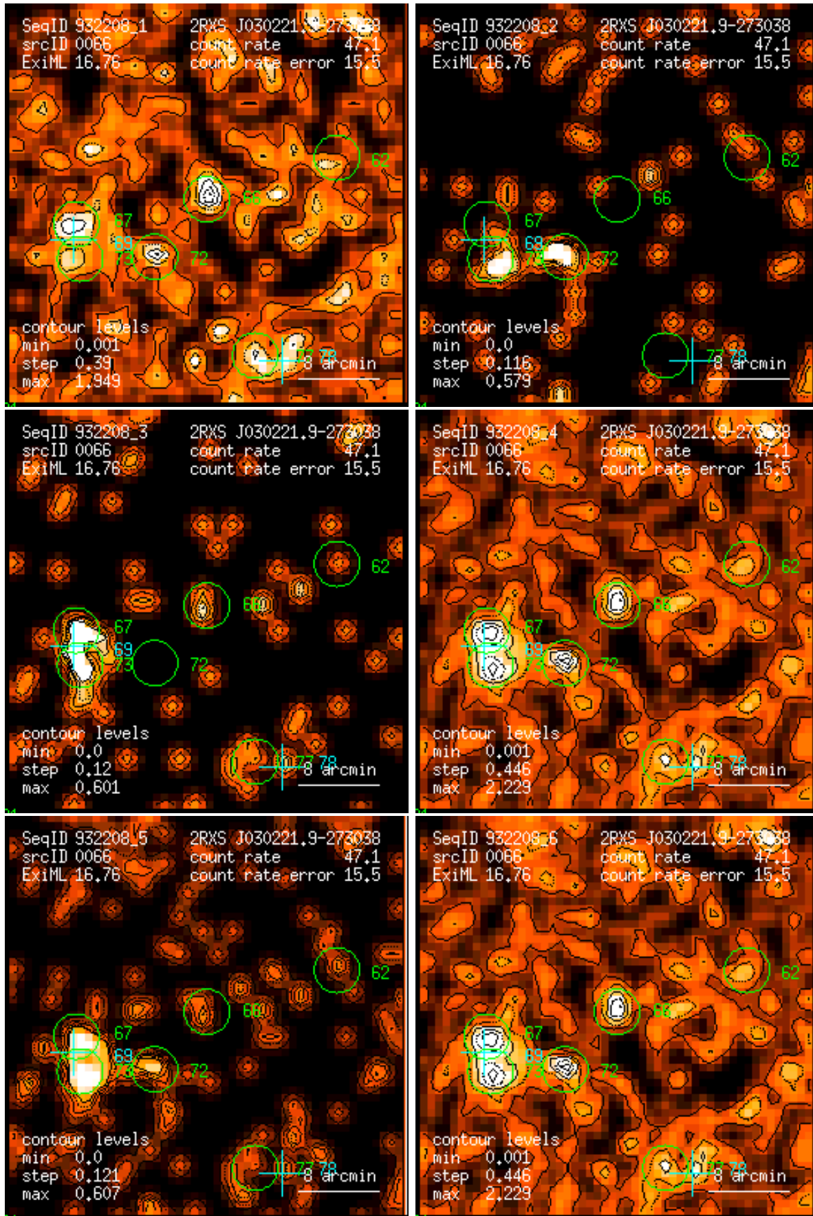
Figure 66: RASS 932208: detection 0066: band rate images, Gaussian filter: (1) PSPC channels 11 – 41, (2) 52 – 90, (3) 91 – 201, (4) 11 – 235, (5) 52 – 201, (6) 11 – 201. Broad band rates in counts/ks. Band rate contour levels in counts/ks/arcmin 2 .
