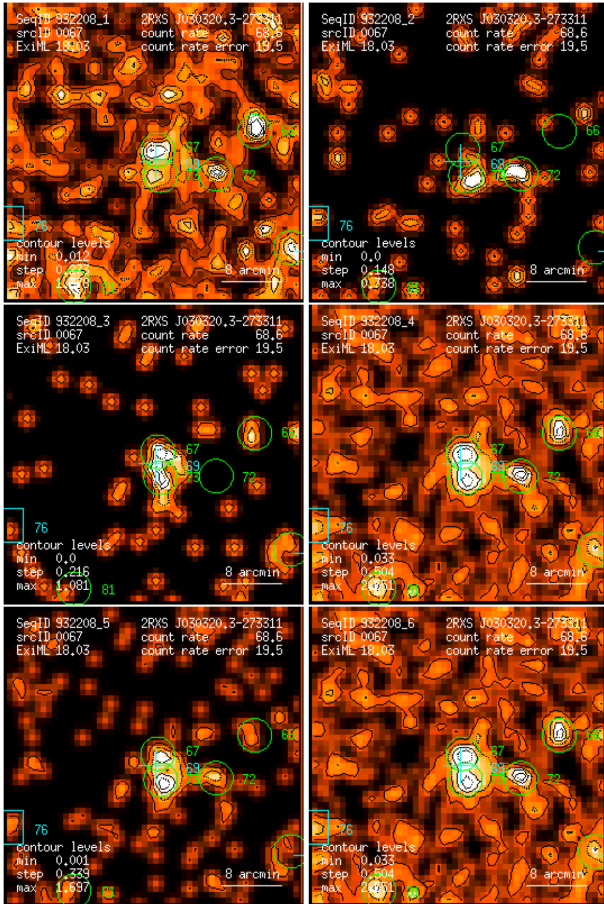
Figure 67: RASS 932208: detection 0067: band rate images, Gaussian filter: (1) PSPC channels 11 – 41, (2) 52 – 90, (3) 91 – 201, (4) 11 – 235, (5) 52 – 201, (6) 11 – 201. Broad band rates in counts/ks. Band rate contour levels in counts/ks/arcmin 2 .
