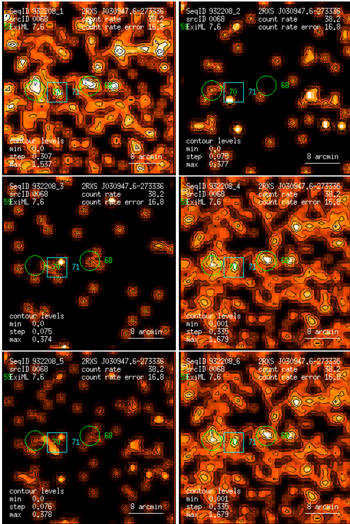
Figure 68: RASS 932208: detection 0068: band rate images, Gaussian filter: (1) PSPC channels 11 – 41, (2) 52 – 90, (3) 91 – 201, (4) 11 – 235, (5) 52 – 201, (6) 11 – 201. Broad band rates in counts/ks. Band rate contour levels in counts/ks/arcmin 2 .
