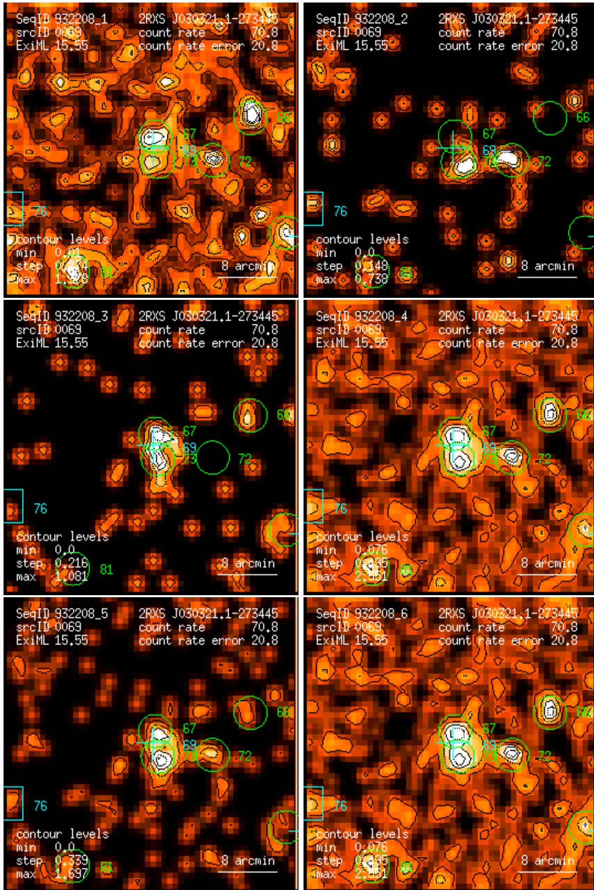
Figure 69: RASS 932208: detection 0069: band rate images, Gaussian filter: (1) PSPC channels 11 – 41, (2) 52 – 90, (3) 91 – 201, (4) 11 – 235, (5) 52 – 201, (6) 11 – 201. Broad band rates in counts/ks. Band rate contour levels in counts/ks/arcmin 2 .
