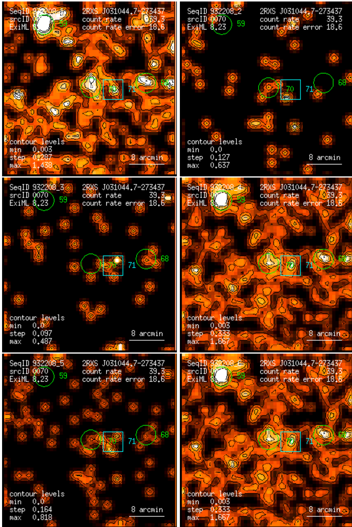
Figure 70: RASS 932208: detection 0070: band rate images, Gaussian filter: (1) PSPC channels 11 – 41, (2) 52 – 90, (3) 91 – 201, (4) 11 – 235, (5) 52 – 201, (6) 11 – 201. Broad band rates in counts/ks. Band rate contour levels in counts/ks/arcmin 2 .
