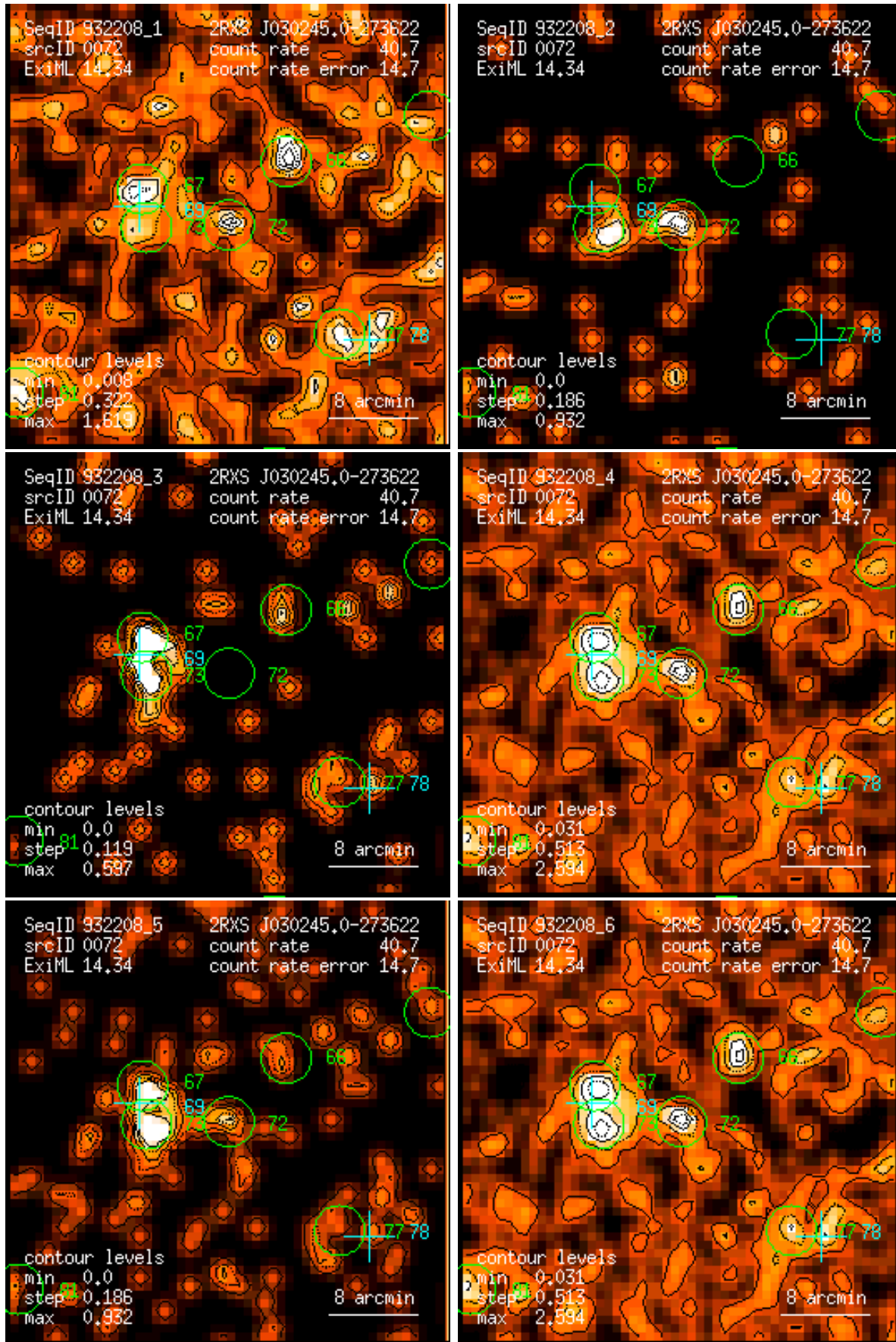
Figure 72: RASS 932208: detection 0072: band rate images, Gaussian filter: (1) PSPC channels 11 – 41, (2) 52 – 90, (3) 91 – 201, (4) 11 – 235, (5) 52 – 201, (6) 11 – 201. Broad band rates in counts/ks. Band rate contour levels in counts/ks/arcmin 2 .
