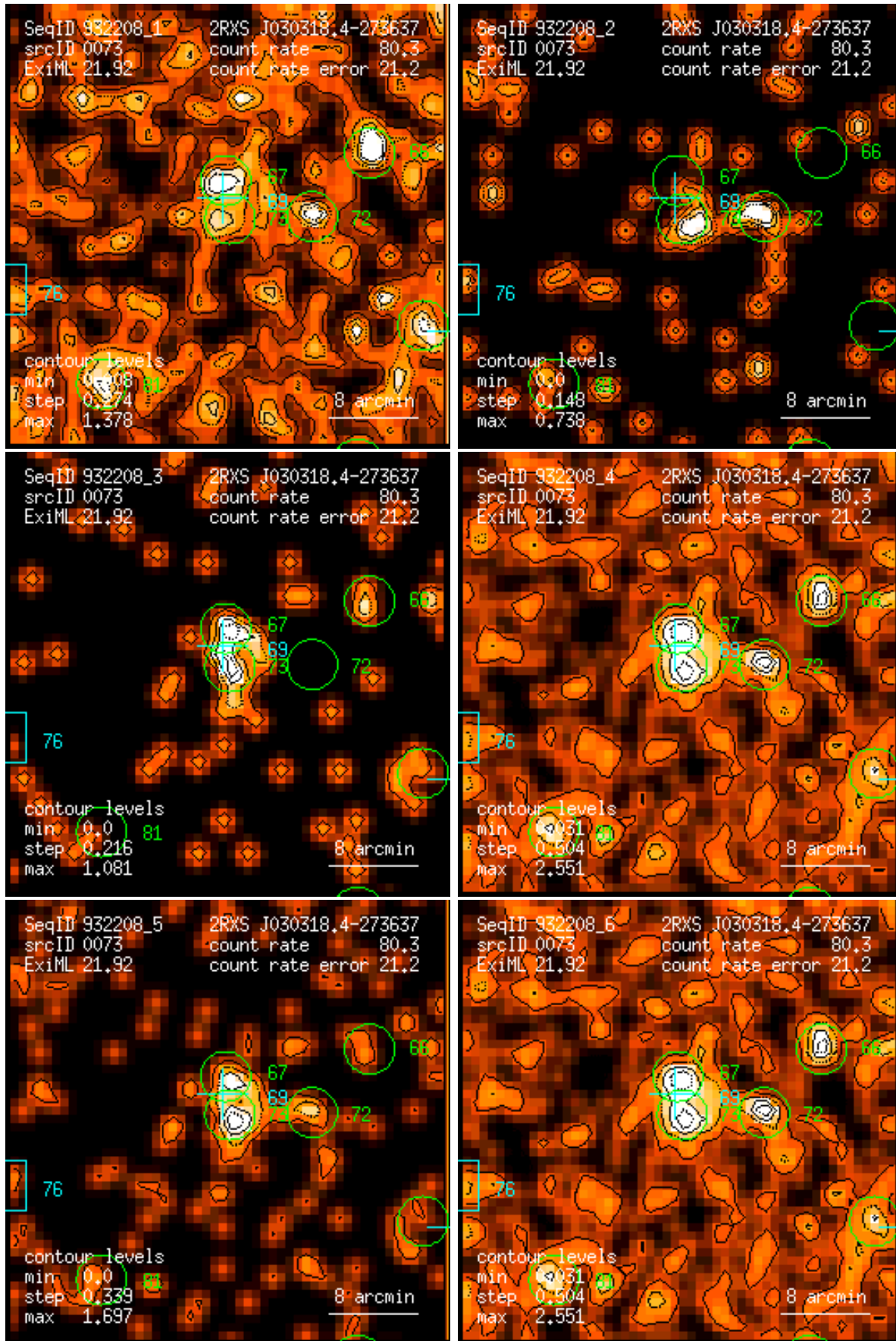
Figure 73: RASS 932208: detection 0073: band rate images, Gaussian filter: (1) PSPC channels 11 – 41, (2) 52 – 90, (3) 91 – 201, (4) 11 – 235, (5) 52 – 201, (6) 11 – 201. Broad band rates in counts/ks. Band rate contour levels in counts/ks/arcmin 2 .
