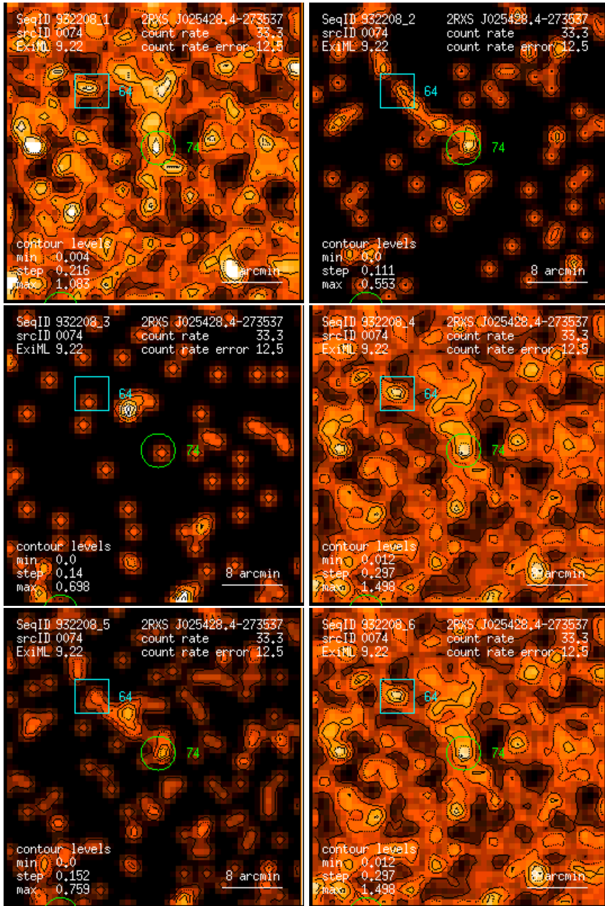
Figure 74: RASS 932208: detection 0074: band rate images, Gaussian filter: (1) PSPC channels 11 – 41, (2) 52 – 90, (3) 91 – 201, (4) 11 – 235, (5) 52 – 201, (6) 11 – 201. Broad band rates in counts/ks. Band rate contour levels in counts/ks/arcmin 2 .
