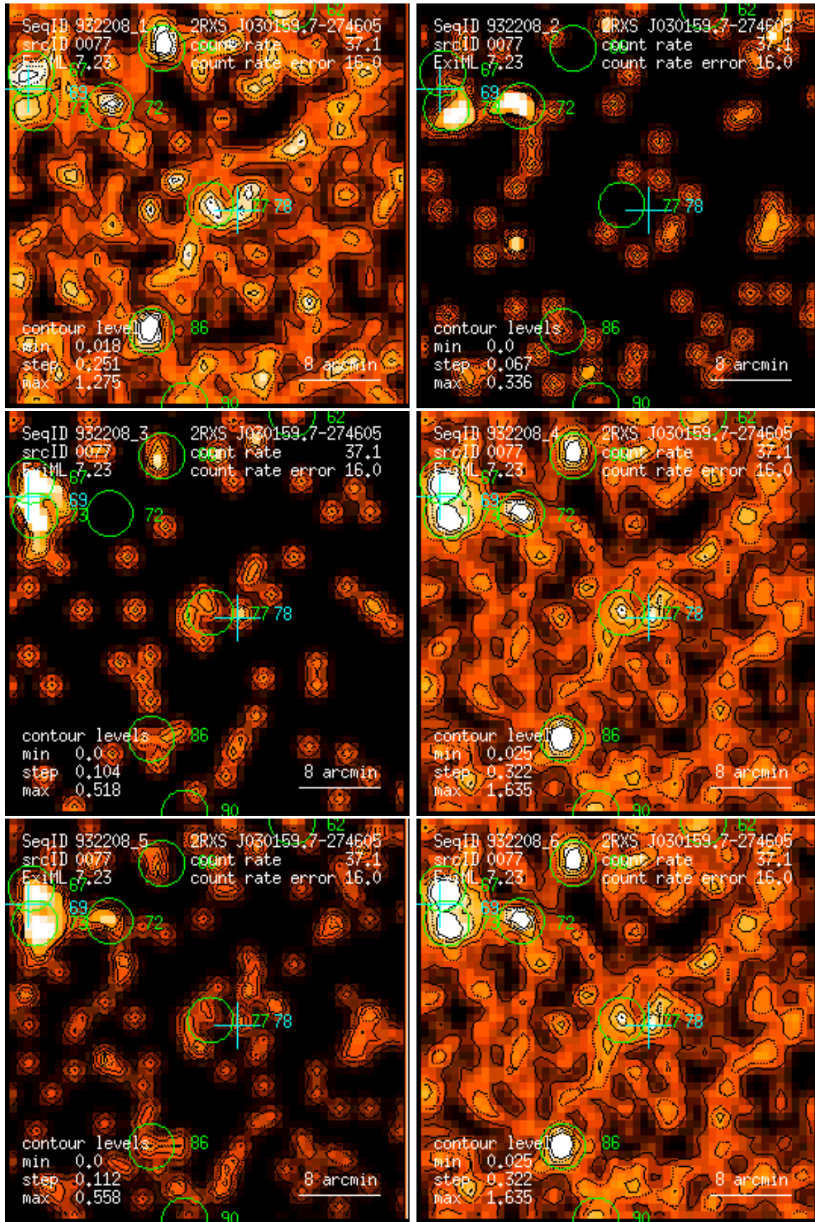
Figure 77: RASS 932208: detection 0077: band rate images, Gaussian filter: (1) PSPC channels 11 – 41, (2) 52 – 90, (3) 91 – 201, (4) 11 – 235, (5) 52 – 201, (6) 11 – 201. Broad band rates in counts/ks. Band rate contour levels in counts/ks/arcmin 2 .
