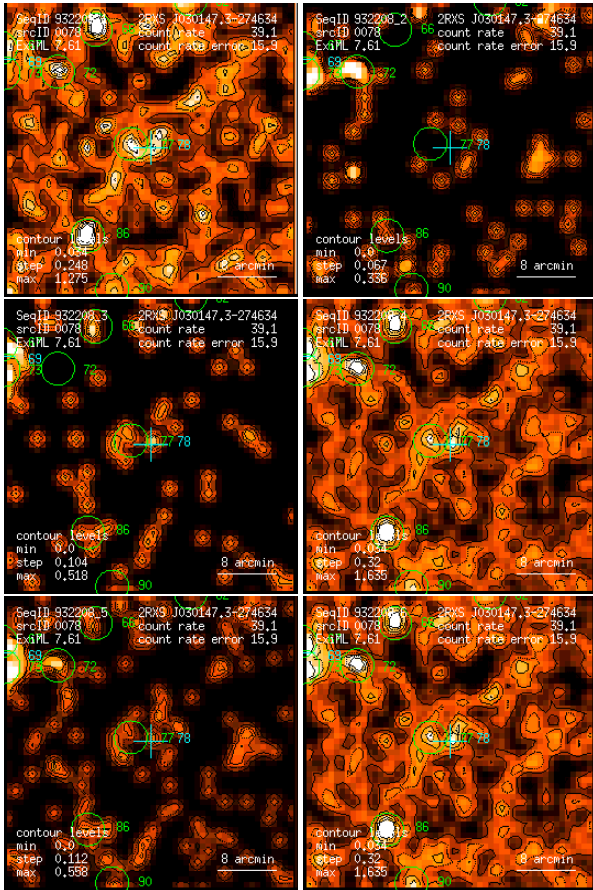
Figure 78: RASS 932208: detection 0078: band rate images, Gaussian filter: (1) PSPC channels 11 – 41, (2) 52 – 90, (3) 91 – 201, (4) 11 – 235, (5) 52 – 201, (6) 11 – 201. Broad band rates in counts/ks. Band rate contour levels in counts/ks/arcmin 2 .
