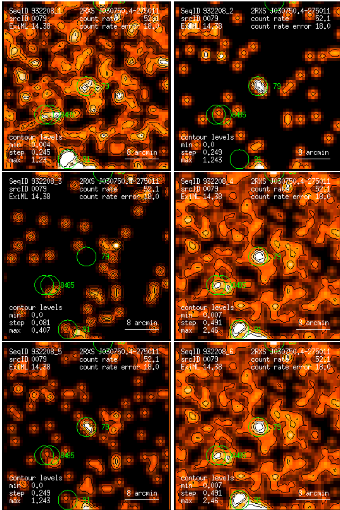
Figure 79: RASS 932208: detection 0079: band rate images, Gaussian filter: (1) PSPC channels 11 – 41, (2) 52 – 90, (3) 91 – 201, (4) 11 – 235, (5) 52 – 201, (6) 11 – 201. Broad band rates in counts/ks. Band rate contour levels in counts/ks/arcmin 2 .
