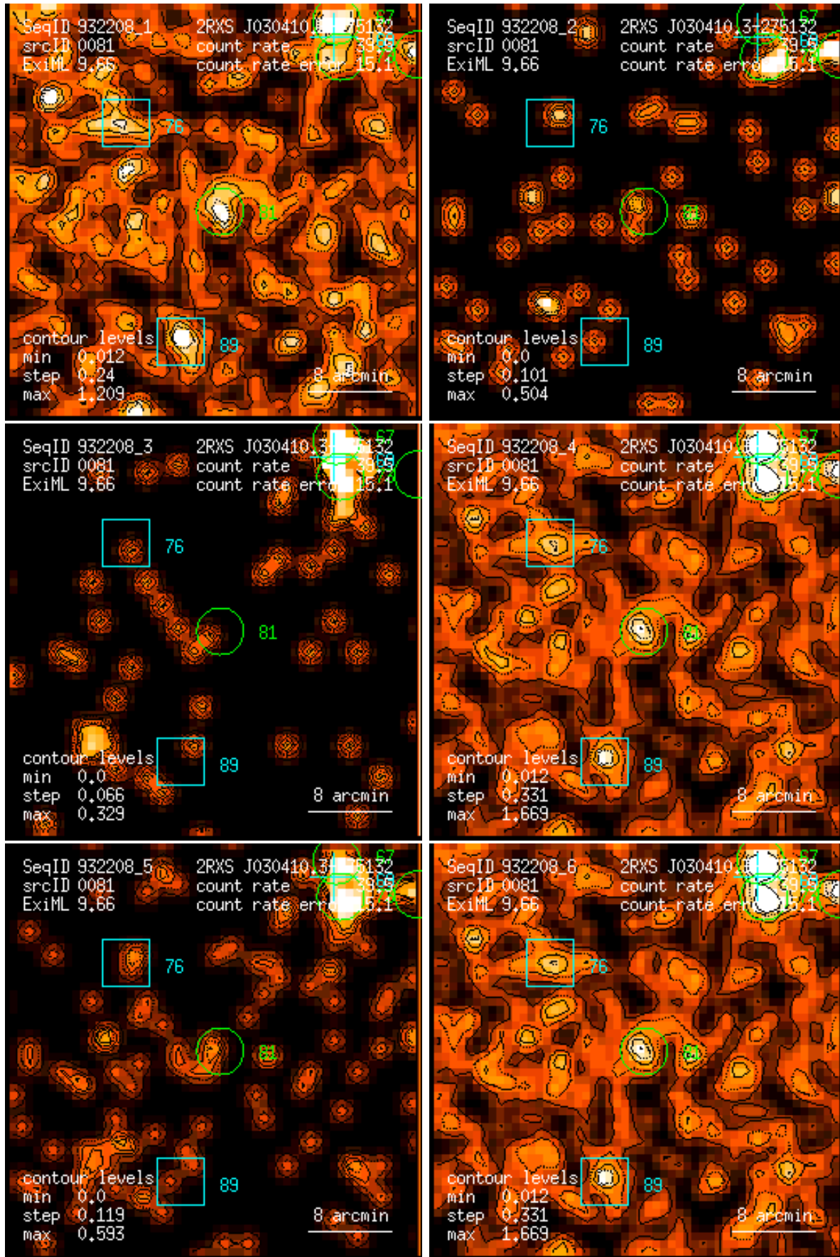
Figure 81: RASS 932208: detection 0081: band rate images, Gaussian filter: (1) PSPC channels 11 – 41, (2) 52 – 90, (3) 91 – 201, (4) 11 – 235, (5) 52 – 201, (6) 11 – 201. Broad band rates in counts/ks. Band rate contour levels in counts/ks/arcmin 2 .
