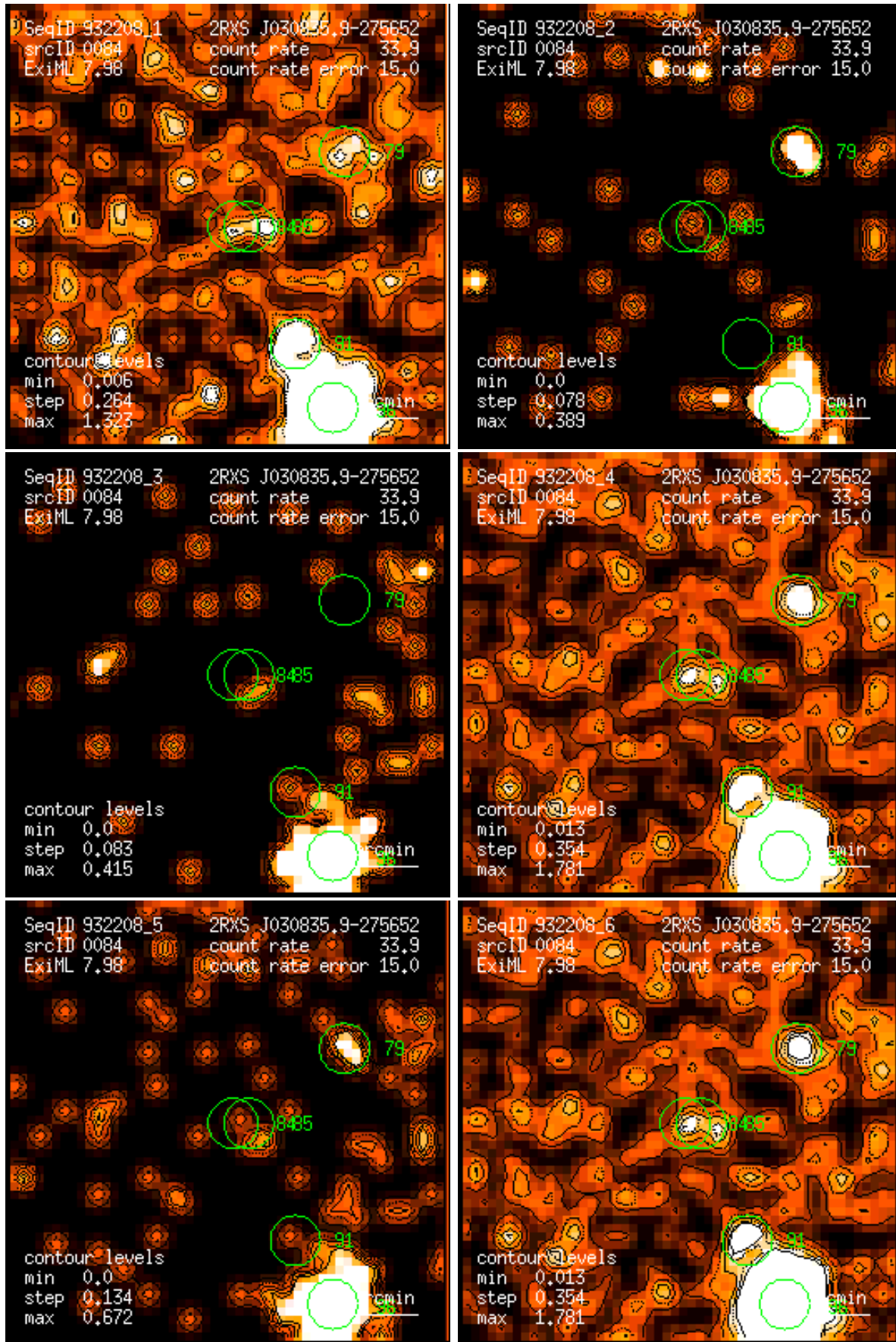
Figure 84: RASS 932208: detection 0084: band rate images, Gaussian filter: (1) PSPC channels 11 – 41, (2) 52 – 90, (3) 91 – 201, (4) 11 – 235, (5) 52 – 201, (6) 11 – 201. Broad band rates in counts/ks. Band rate contour levels in counts/ks/arcmin 2 .
