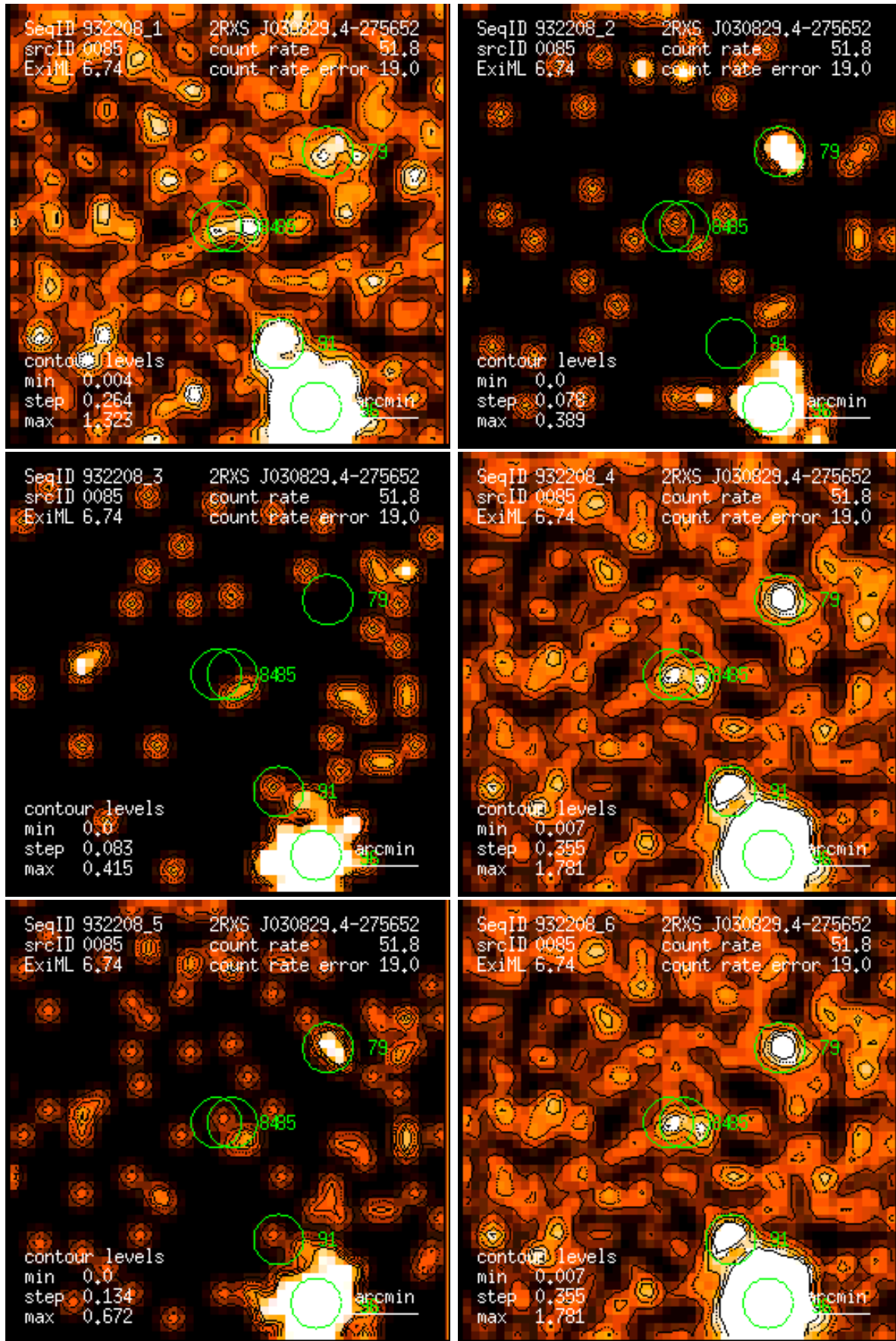
Figure 85: RASS 932208: detection 0085: band rate images, Gaussian filter: (1) PSPC channels 11 – 41, (2) 52 – 90, (3) 91 – 201, (4) 11 – 235, (5) 52 – 201, (6) 11 – 201. Broad band rates in counts/ks. Band rate contour levels in counts/ks/arcmin 2 .
