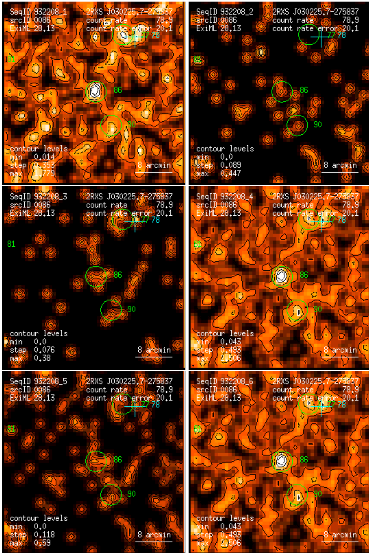
Figure 86: RASS 932208: detection 0086: band rate images, Gaussian filter: (1) PSPC channels 11 – 41, (2) 52 – 90, (3) 91 – 201, (4) 11 – 235, (5) 52 – 201, (6) 11 – 201. Broad band rates in counts/ks. Band rate contour levels in counts/ks/arcmin 2 .
