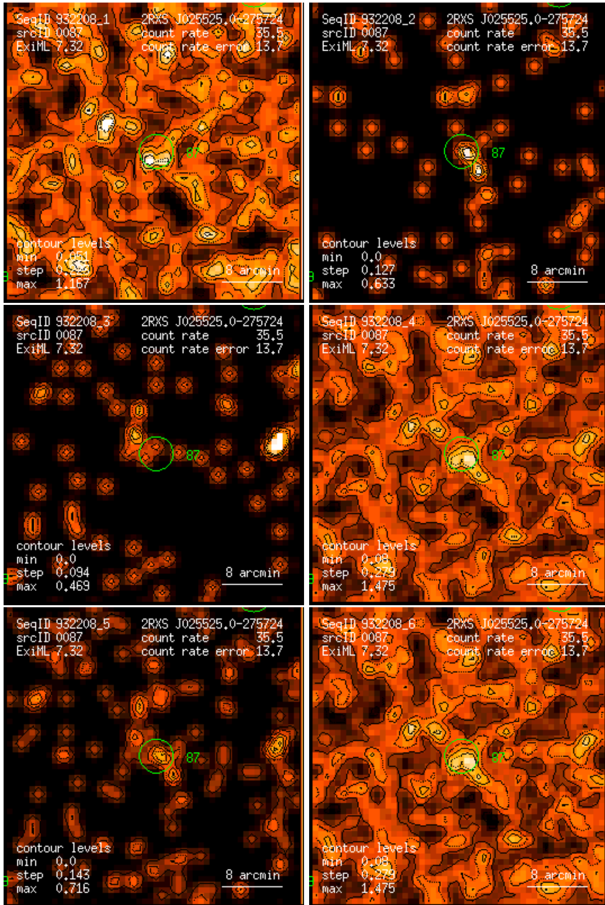
Figure 87: RASS 932208: detection 0087: band rate images, Gaussian filter: (1) PSPC channels 11 – 41, (2) 52 – 90, (3) 91 – 201, (4) 11 – 235, (5) 52 – 201, (6) 11 – 201. Broad band rates in counts/ks. Band rate contour levels in counts/ks/arcmin 2 .
